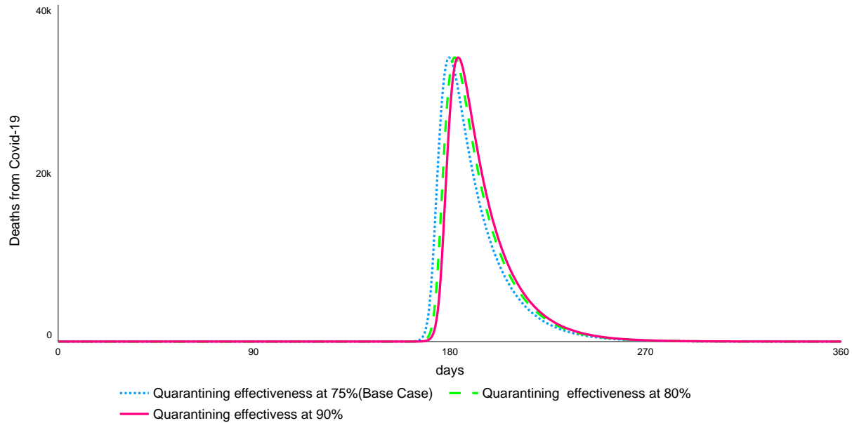
Fig 9b. Impact of varying levels of quarantining effectiveness on Covid-19 deaths
