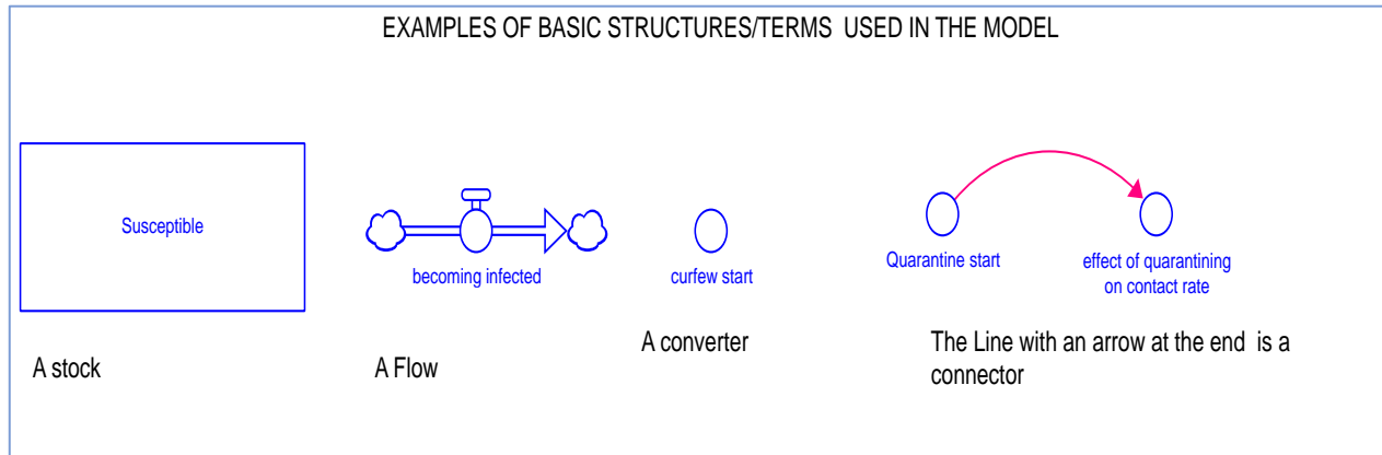
Figure 1: Basic structures and terms used in SDM
