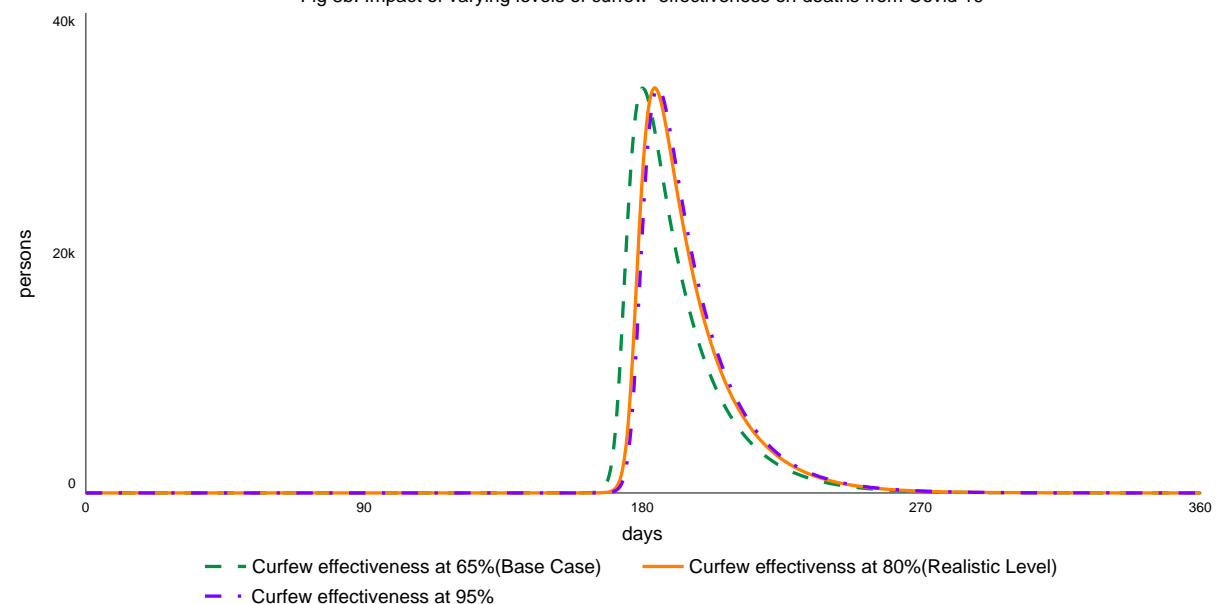
Fig 8b. Impact of varying levels of curfew effectiveness on deaths from Covid 19
