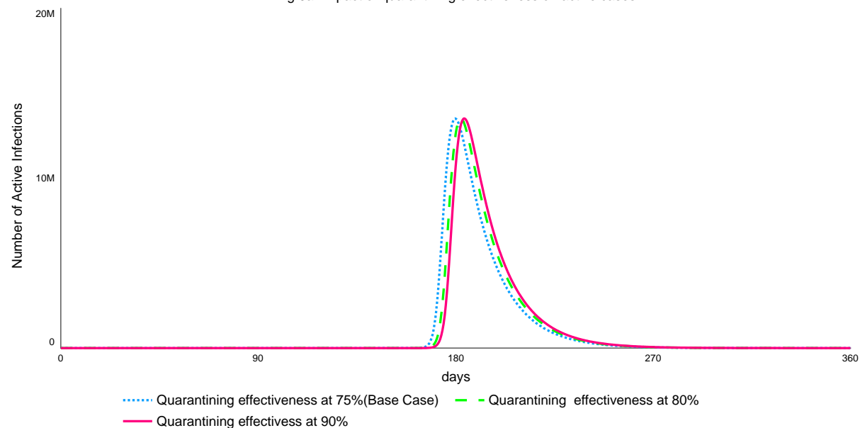
Fig 9a. Impact of quarantining effectiveness on active cases
