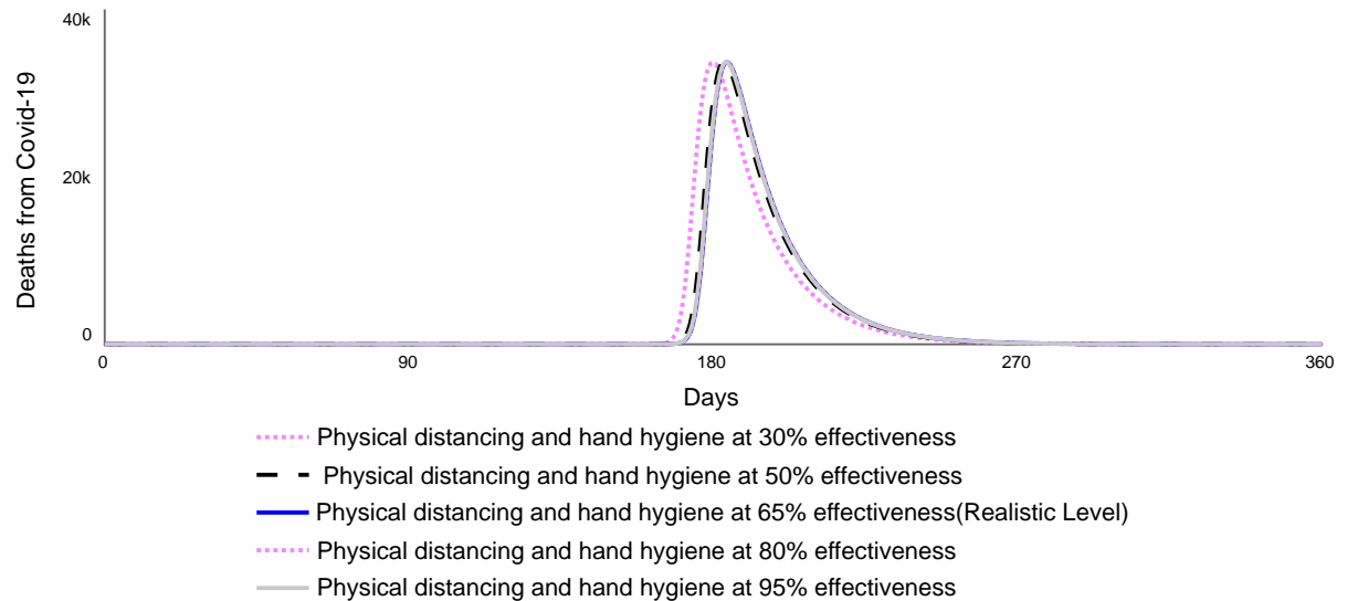
Fig 7b. Impact of Physical distancing and hand Hygiene on Mortality
