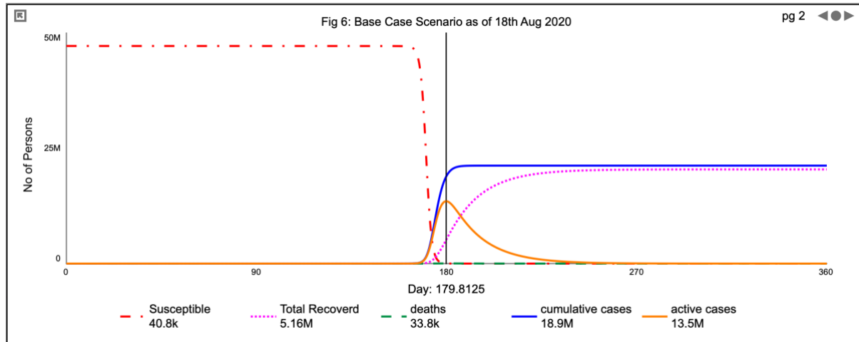
Figure 6. Base Case scenario of Covid-19 possible trajectory in Kenya as of 18 th August 2020.
