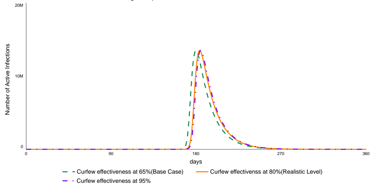
Fig 8a. Impact of curfew effectiveness on active cases
