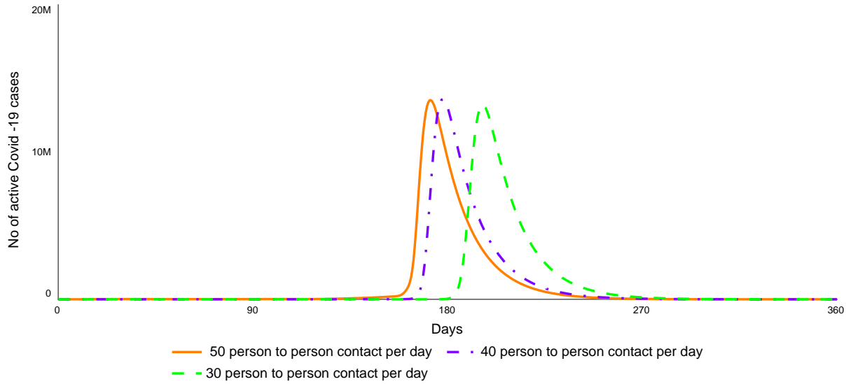
Fig 10 : Impact of person to person contact on the number of active cases
