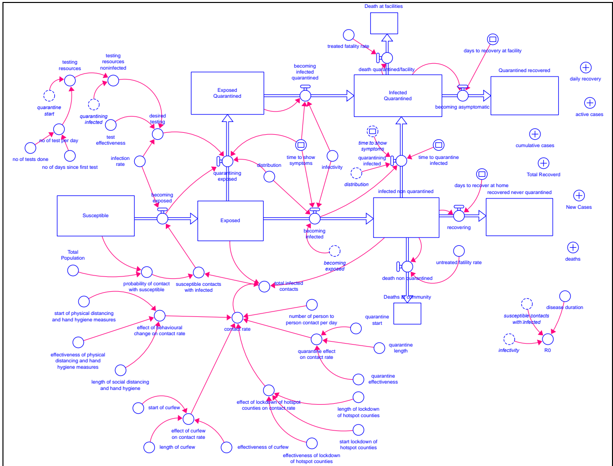
Fig 2: Overview of Stock and Flow diagram of Covid-19 trajectory in Kenya.
