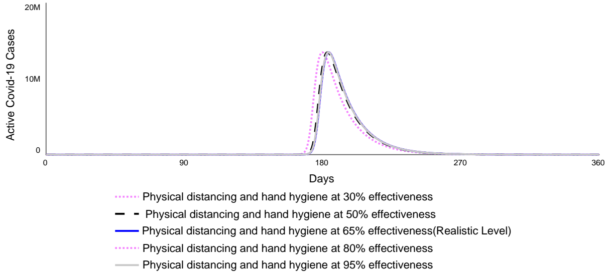
Fig 7a. Impact of Physical Distancing and Hand Hygiene on Active cases
