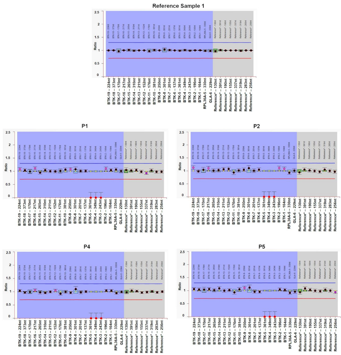
Figure 2: Multiplex ligation dependent amplification (MLPA) assay for detection of deletion 3-5 exons of the BTK gene: Representation of ratio charts generated using the Coffalyser.net software. (A) Reference sample depicts the normal copies of the BTK gene and other samples (B) Sample P1 (C) Sample P2 (D) Sample P4 (E) Sample P5 are all males and depict probe ratio of zero for 3-5 exons of the BTK gene which lies on X-chromosome, i.e. they have hemizygous deletion. For all the ratio charts, the
