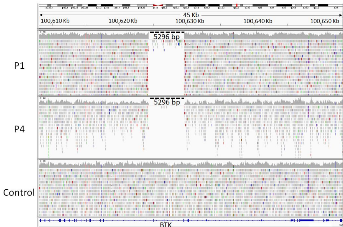
Figure 1: Identification of putative large deletion in whole genome data in P1 and P4: The figure represents the visualization of sequencing reads aligned on the coding region of the BTK gene.
