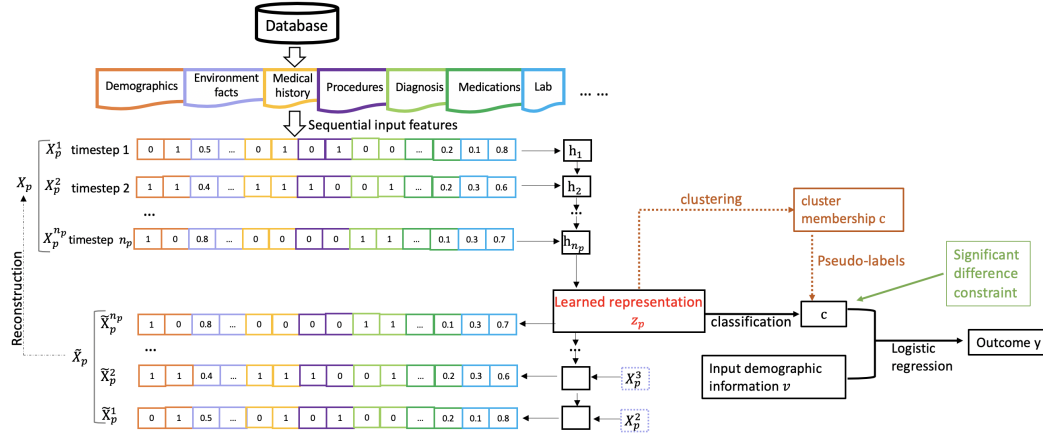
Figure 1: The framework of the proposed deep significance clustering (DICE). Clustering is applied to the representation \mathbf{z}_p . A statistical significance constraint is explicitly added to ensure the association of the clustering membership \mathbf{c} and outcome y to facilitate the learning of discriminative representations \mathbf{z}_p .
