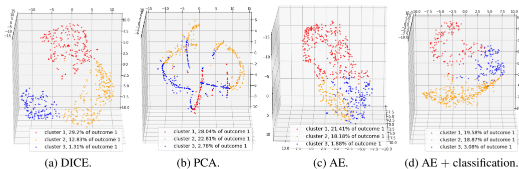
Figure 4: Visualization of patient subtyping results by various methods on COVID-19 dataset.
