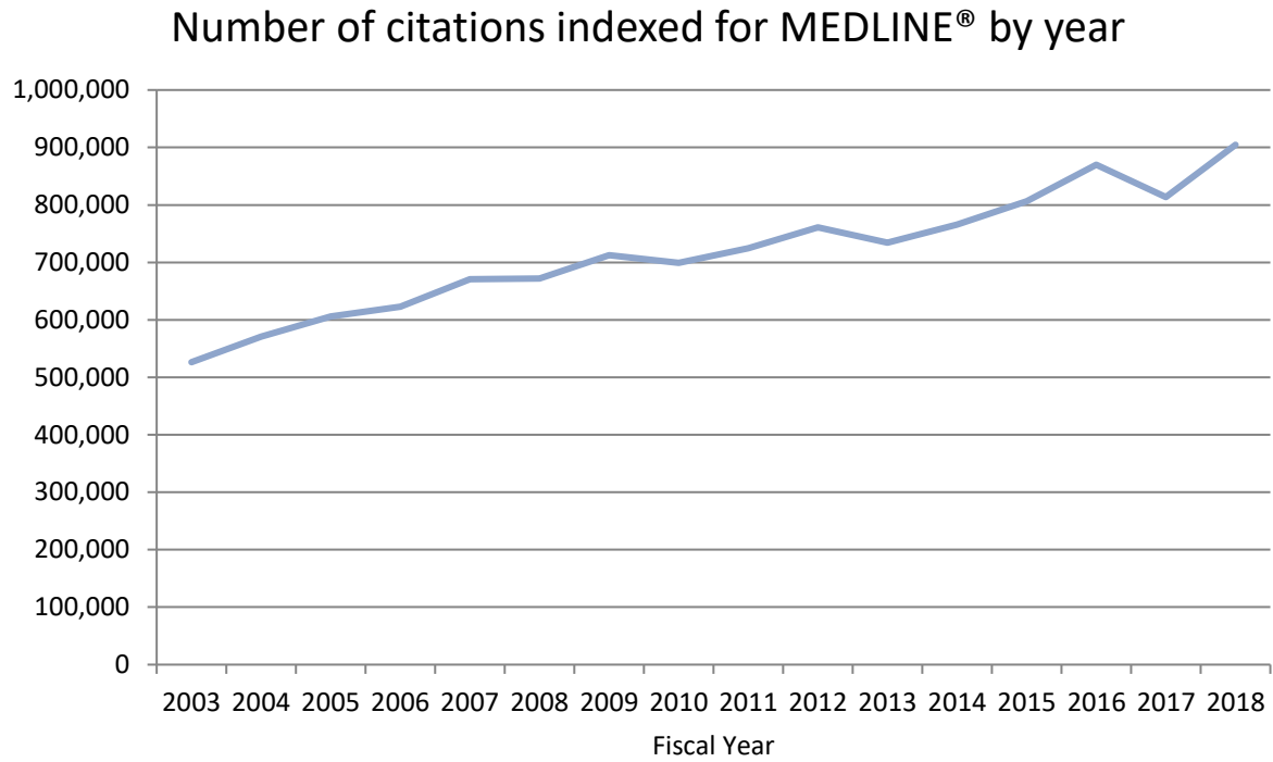
Figure 3. The number of citations indexed for MEDLINE® each year [Data from NLM website URL https://www.nlm.nih.gov/bsd/bsd_key.html ]
