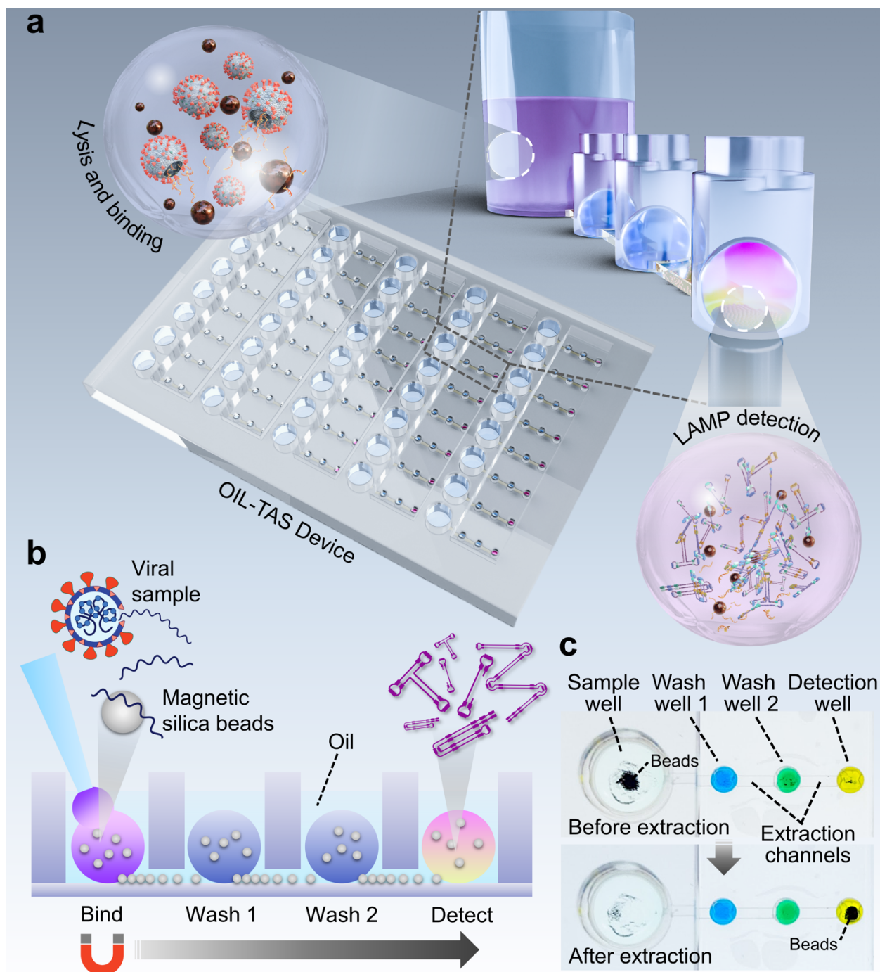
Fig. 1 Integrated RNA extraction and detection with the OIL-TAS platform. a Schematic depicting the design and essential components of the OIL-TAS. b Side view cartoon illustrating the operation principle of OIL-TAS sample extraction. Owing to the exclusive liquid repellent (ELR) nature of the device surface, droplets appear spherical which minimizes contact with the device surface and hence biofouling associated sample loss. c Images of a single unit of the OIL-TAS device before and after extraction. Each unit includes a large sample well for sample lysis and binding, followed by two washing wells and a detection well. Interconnecting the wells are oil-filled extraction channels. Wells are filled with droplets of food coloring for visualization.
