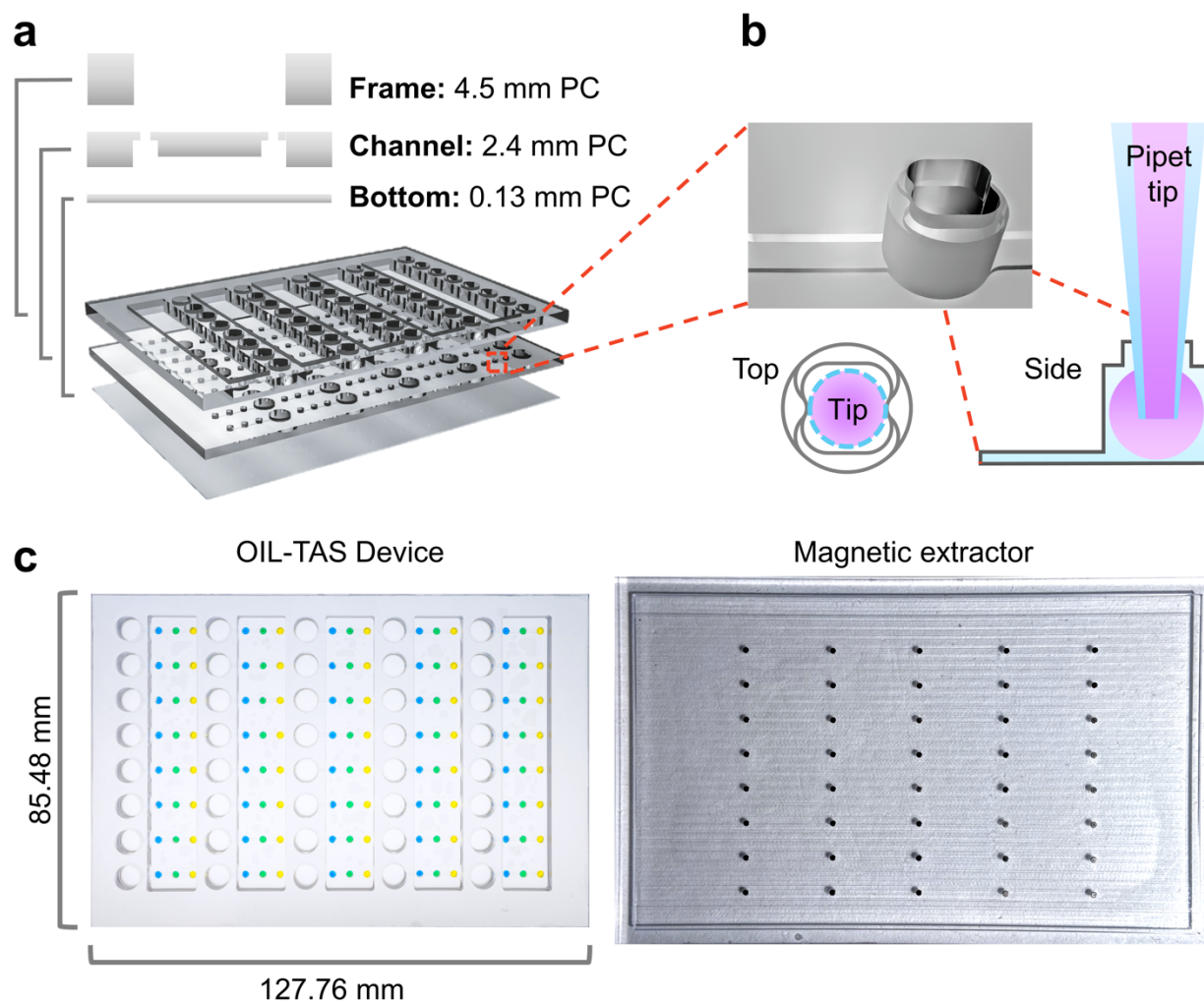
Fig. 2 Design and assembly of the OIL-TAS device. a Exploded view of the OIL-TAS device consisting of 3 layers fabricated from polycarbonate (PC). b Design of well collar for pipet tip alignment and preventing droplet escape. c Images of OIL-TAS device (left) and magnetic extractor (right). Food coloring was added to the wells to facilitate visualization.
