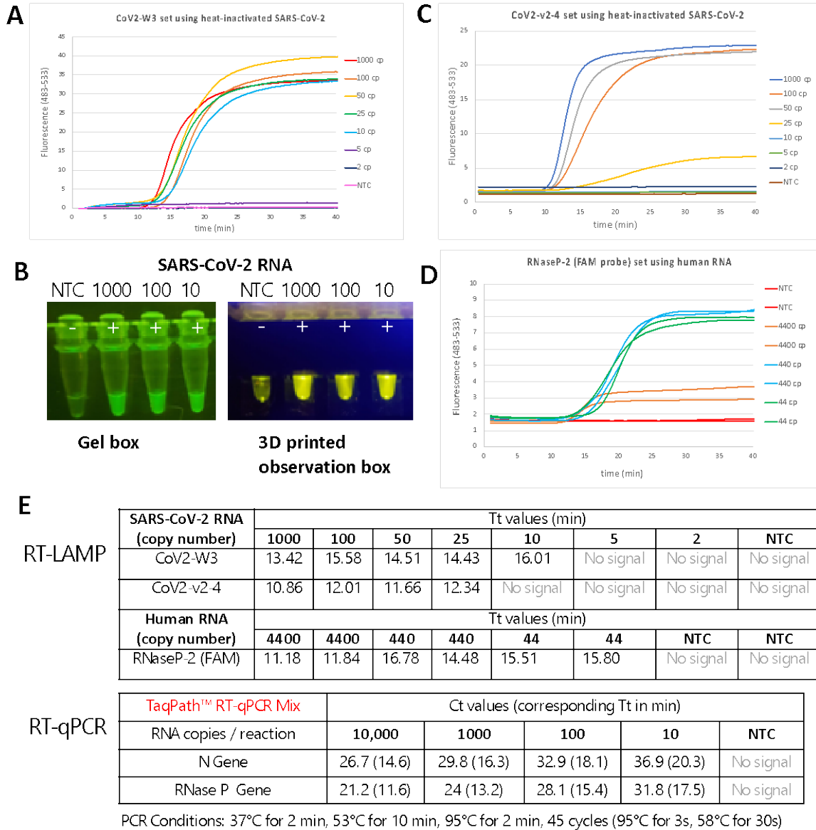
Fig 2. Limit of detection using DP-RT-LAMP primers using heat-inactivated SARS-COV-2 or human RNA (for internal control).
