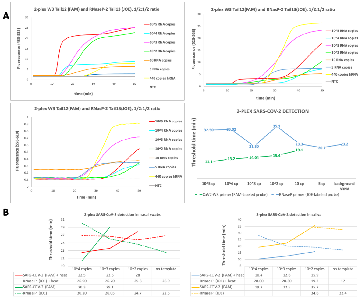
Fig 6. Multiplexed detection of SARS-COV-2 RNA and RNase P (internal control).
