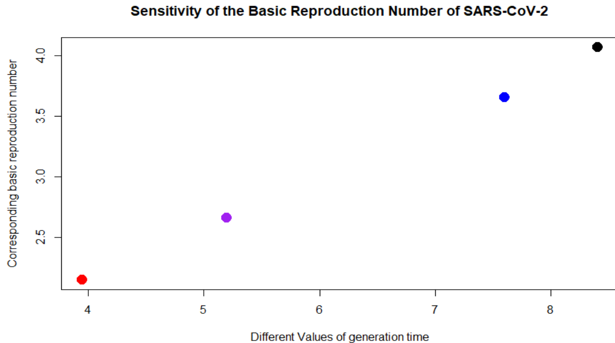
Figure 1. Different values of R_0 corresponding to different values of generation time is illustrated. The values of R_0 corresponding to generation time 3.95, 5.20, 7.60, and 8.40 represented by red, purple, blue, and black dots, respectively.
