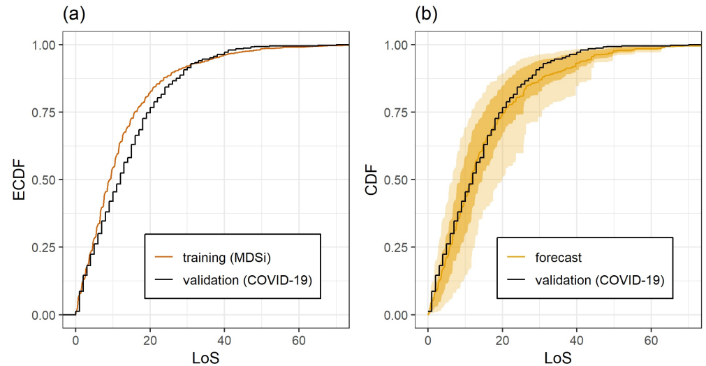
Fig 2. (a) Empirical distributions of LoS in training and validation dataset. (b) Empirical CDF of the LoS in the validation dataset (black stepfunction) and average LoS forecasts for the COVID-19 patients (orange curve). Shaded areas show the pointwise 25% and 75% (10% and 90% for the outer bounds) quantiles of the predictive CDFs.
