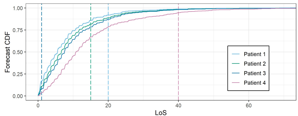
Fig 1. Predictive CDFs for the LoS of some COVID-19 patients with corresponding realizations as a vertical line.
