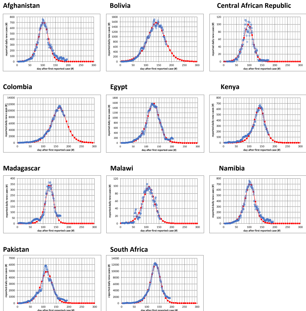
Figure 2. COVID-19 reported cases in 11 selected low- and middle-income countries, together with best-fit curves from simple disease spread model. Blue circles show daily reported new cases of COVID-19 (based on a 7-day rolling average). Red squares (joined by straight lines) show best-fit outputs from linearized Reed-Frost model.
