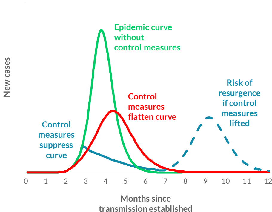
Figure 1. Typical disease outbreak curves in different scenarios. 1
