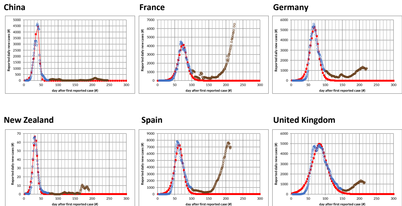
Figure 3. COVID-19 reported cases in 6 selected comparison countries, together with best-fit curves from test of simple disease outbreak model. Blue and brown circles show daily reported new cases of COVID-19 (based on a 7-day rolling average). Red squares (joined by straight lines) show best-fit outputs from linearized Reed-Frost model, fit only to the blue circles in the first peaks in cases.
