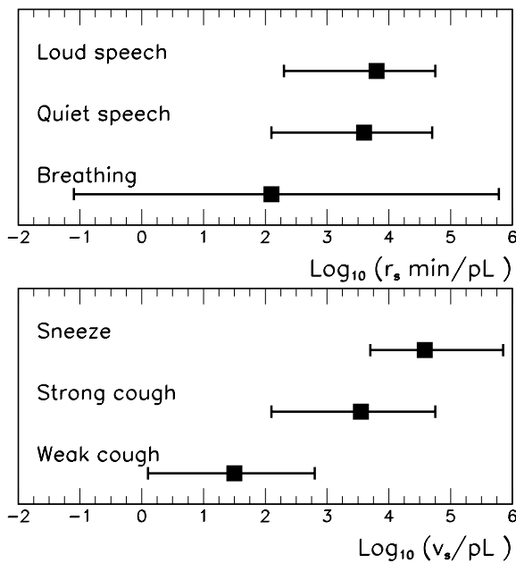
FIG. 1: Box-whisker chart of the emission aerosol rate r_s and the total aerosol volume v_s that are expelled by a source s .
