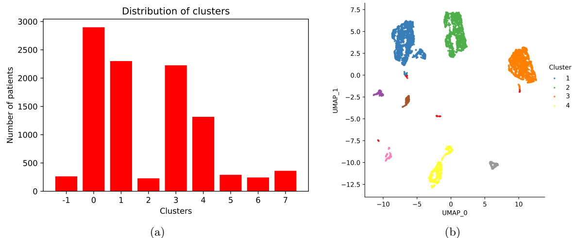
Figure 3: (a) Distribution of clusters detected by DBSCAN on the five dimensional reduced representation of the data (b) UMAP clusters for five dimensional reduced representation of the data annotated by the DBSCAN generated clusters
