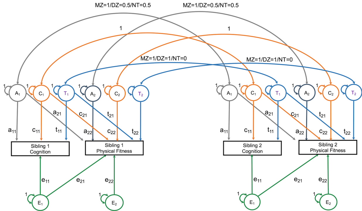
Figure 1: Overview of Bivariate Cholesky Decomposition Model
