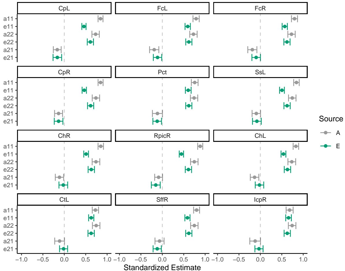
Figure 5: Behavioral genetic path estimates for BMI and white matter FA
