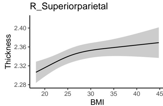
Figure 3: Association between BMI and GM thickness values
