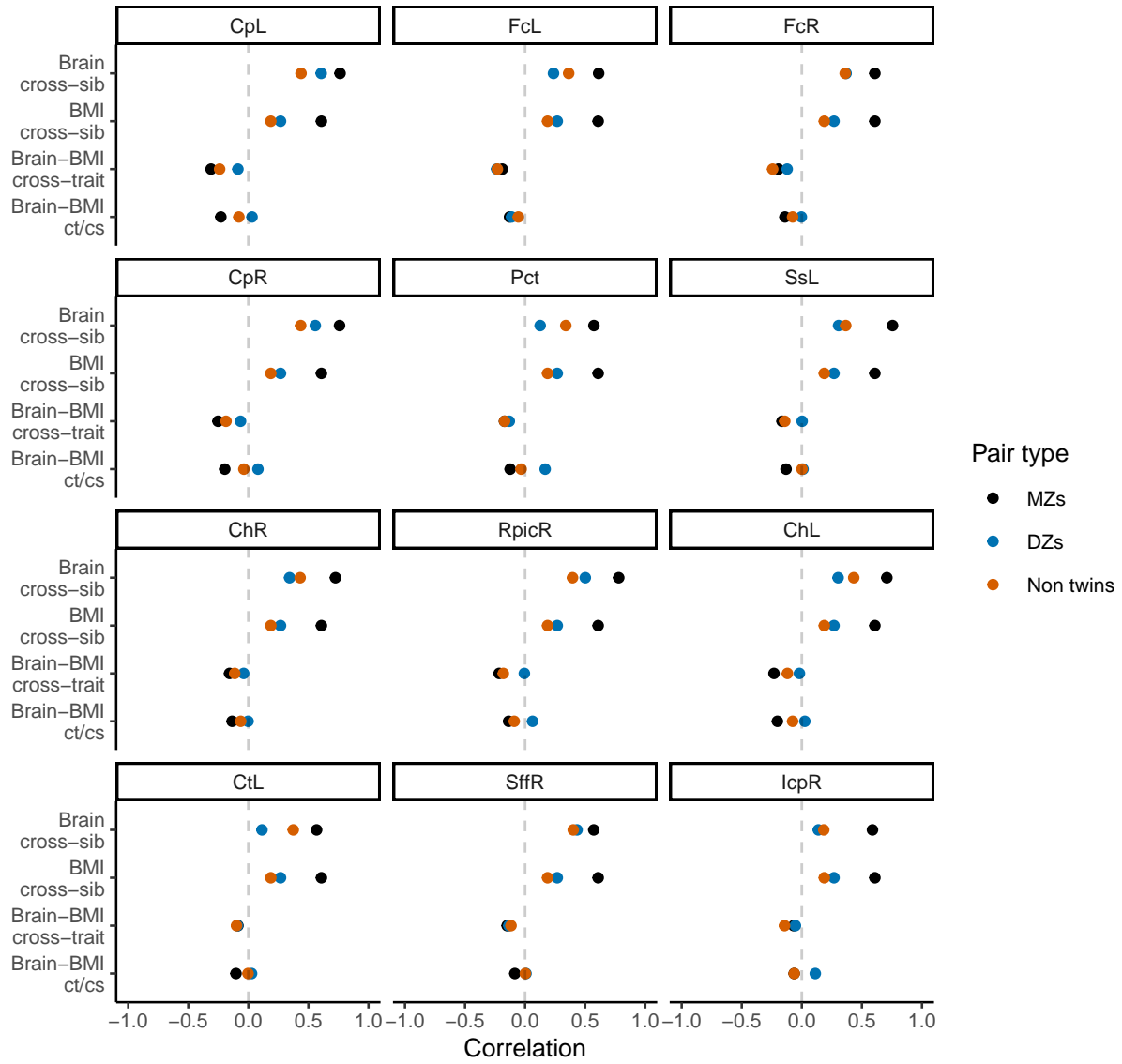
Figure 4: Phenotypic correlations across siblings and across traits
