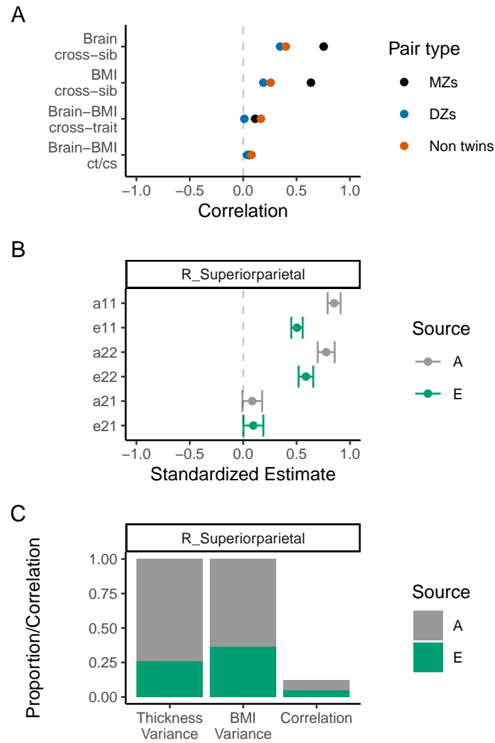
Figure 7: Summary of behavioral genetic analyses of BMI and right superior parietal thickness
