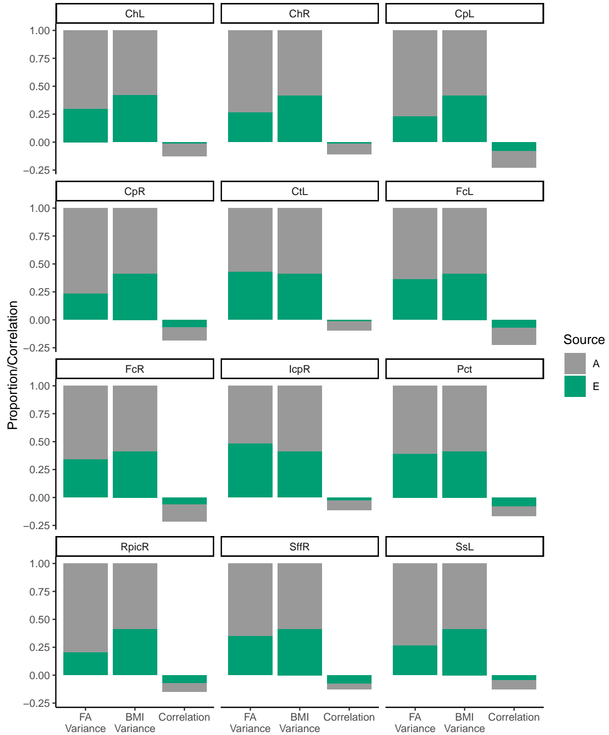
Figure 6: Variance components for BMI and white matter FA
