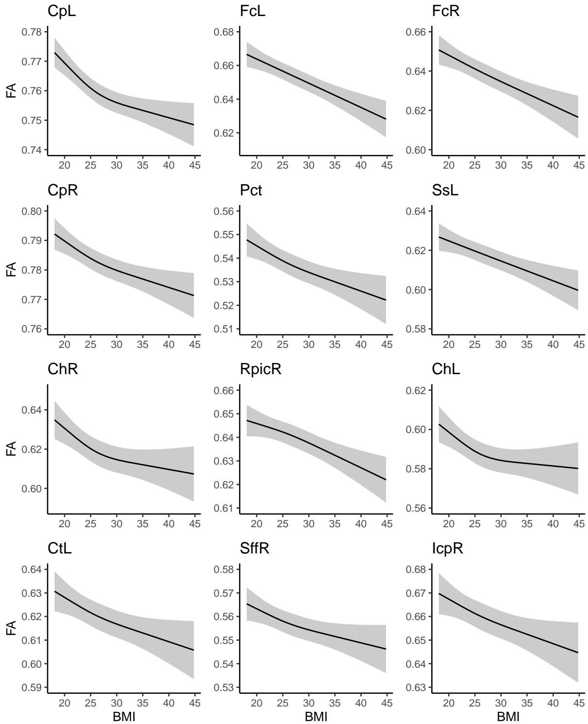
Figure 2: Association between BMI and white matter FA values
