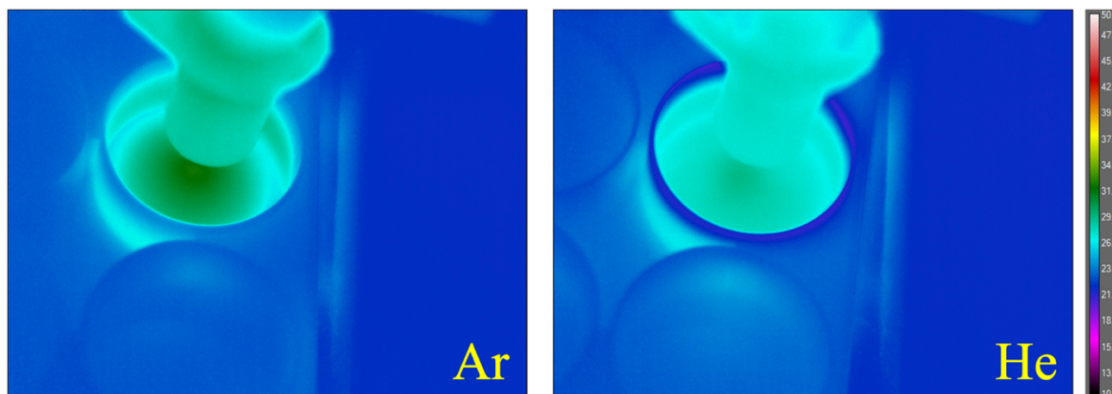
Figure 2. Temperature distribution of Ar and He plasma-treated 6-well plate. The highest temperature for each subject was found at the center of the circular thermal gradient immediately beneath the plasma discharge. The center temperature for the Ar plasma treated surface was approximately 32 °C and for the He plasma treatment was approximately 29 °C.
