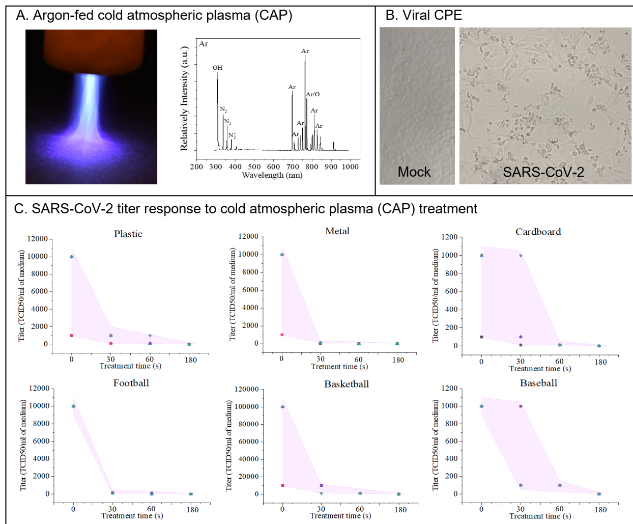
Figure 1. Ar-fed CAP disinfecting SARS-CoV-2. Panel A shows Ar-fed CAP treatment of a plastic surface and the optical emission spectrum of reactive oxygen and nitrogen species (RONS) (Exposure: 250 ms). Panel B shows a Bright-field image of SARS-CoV-2 infected Vero-E6 cells showing viral cytopathic effect (CPE). Uninfected (Mock) cells included as control. Panel C shows SARS-CoV-2 titer response to CAP treatment times of 0, 30, 60, and 180 seconds on surfaces of plastic, metal, cardboard, leather football, composite leather basketball, and leather baseball. Error bar in each graph is shown as shaded area.
