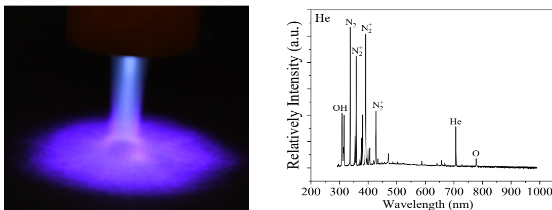
Figure 4. He-fed CAP and its spectrum. Left: He-fed plasma jet treating surface with plume spreading across the surface. Right: The He-fed plasma jet was detected by the optical emission spectrum and contained reactive oxygen and nitrogen species (RONS) (Exposure: 5000 ms).
