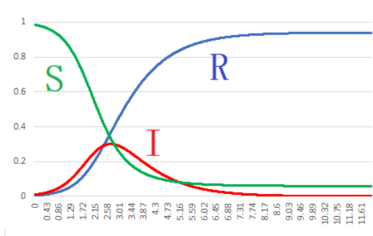
Figure 1: Graph of S , I and R for \alpha = 3 and c = 0.04
