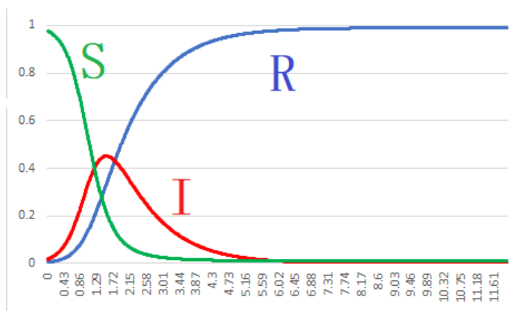
Figure 2: Graph of S , I and R for \alpha = 4.6 and c = 0.028
