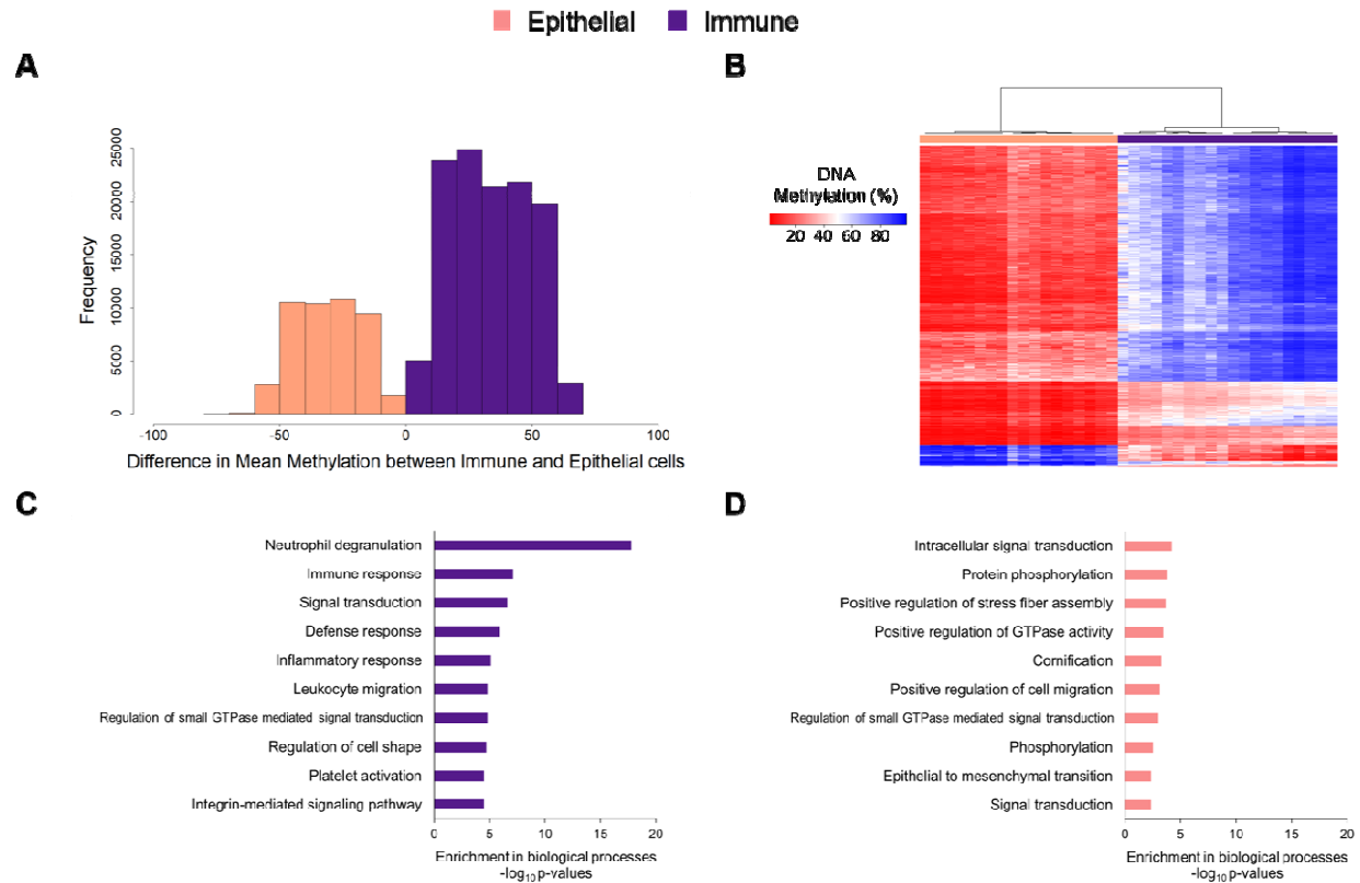
Figure 4. DNA methylation differences between immune and epithelial cell types. A) Among DNA methylation sites differentially methylated between immune and epithelial cells ( p < 10^{-8} , 164,793 sites), histogram of the magnitude of DNA methylation difference. The x-axis is percent methylation, and the reference group was epithelial cells. The values were calculated as percent methylation of immune minus that of epithelial. B) The top 500 most differentially methylated sites between immune and epithelial cells by p-value (t-test) are plotted in heatmap rows (red indicates lower DNA methylation, blue indicates higher DNA methylation). In heatmap columns, unbiased hierarchical clustering of samples was performed (immune fractions in purple and epithelial fractions in pink). C) Bar chart of the gene ontology biological processes enriched (minimum p < 3.2 \times 10^{-5} ) among genes hypomethylated in immune cells, relative to epithelial cells. D) Bar chart of the gene ontology biological processes enriched (minimum p < 4.7 \times 10^{-3} ) among genes hypomethylated in epithelial cells, relative to immune cells.
