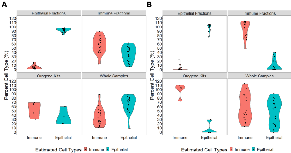
Figure 5. Cell-type percentages estimated in saliva samples from DNA methylation data, using two estimation methods. Violin plots are used to visualize the percent immune cells estimated in red and the percent epithelial cells estimated in blue. In both panels A and B, the upper left quadrant shows the percent cell types estimated in sorted epithelial samples (n=18); the upper right quadrant shows the percent cell types estimated in sorted immune cell samples (n=20), the lower left quadrant shows the percent cell types estimated in whole saliva collected in Oragene kits (n=4); and the lower right quadrant shows the percent cell types estimated in whole saliva samples collected directly (n=18). A) Percent cell types were estimated using a reference panel generated from ENCODE epithelial cell DNA methylation data 29,31 and an adult white blood cell data, 30 implemented through ewastools. B) Percent cell types estimated using our new primary saliva reference panel implemented through ewastools. 23
