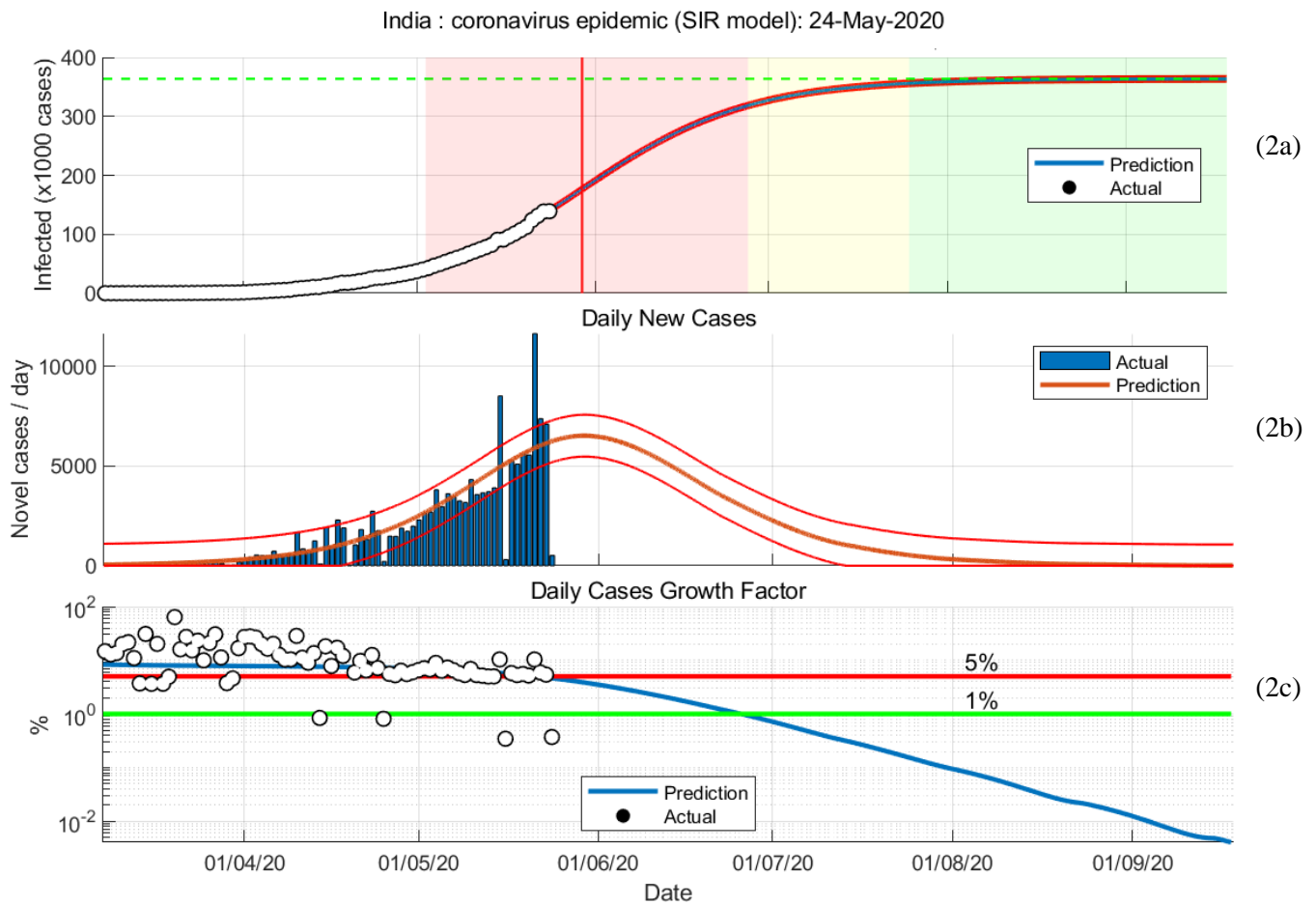
Figure 2: Graphical representations of SIR model 1 30-Jan to 24-May
