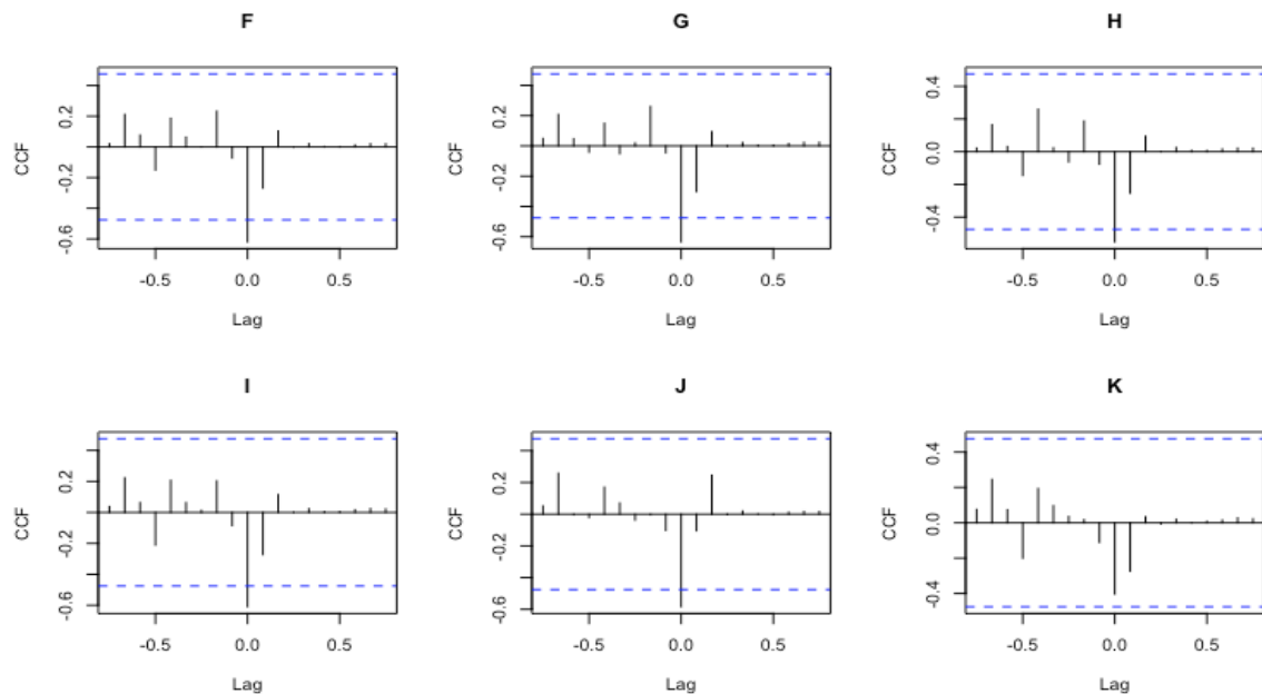
Figure 5. Cross-correlation test for COVID-19 time series and antigens (f) OPV_2, (g) DTP2, (h) OPV3, (i) IPV, (j) Td1, (k) Td2+
