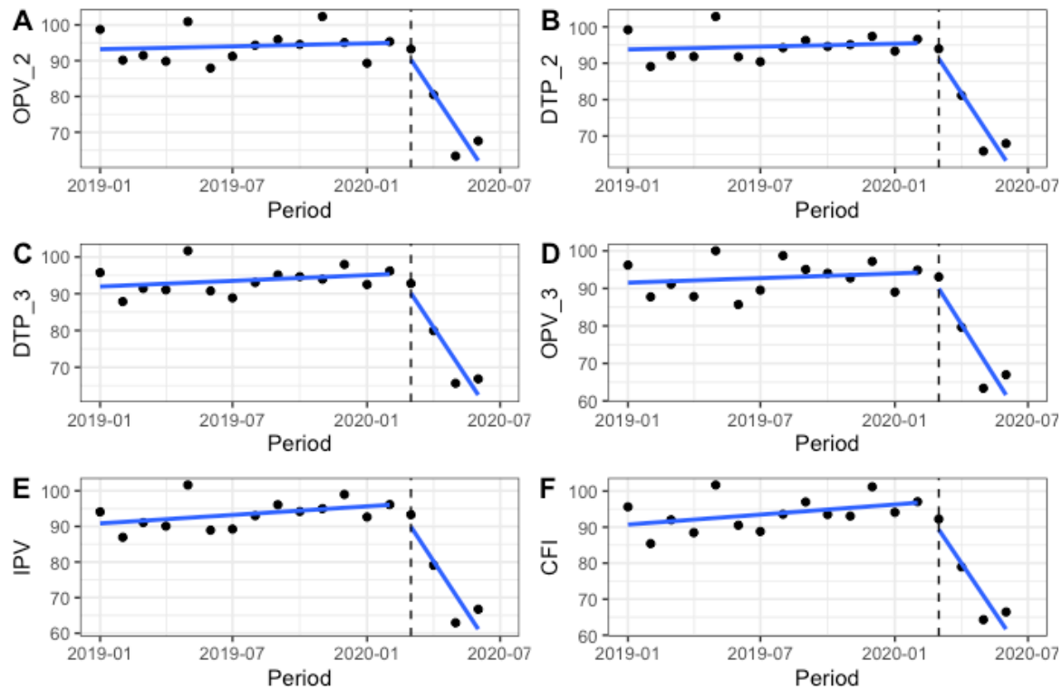
Figure 2. Trends in vaccine coverage of antigens (a) OPV_2, (b) DTP2, (c) DTP3, and (d) OPV3, (e) IPV, (f) Children fully vaccinated (CFI)
