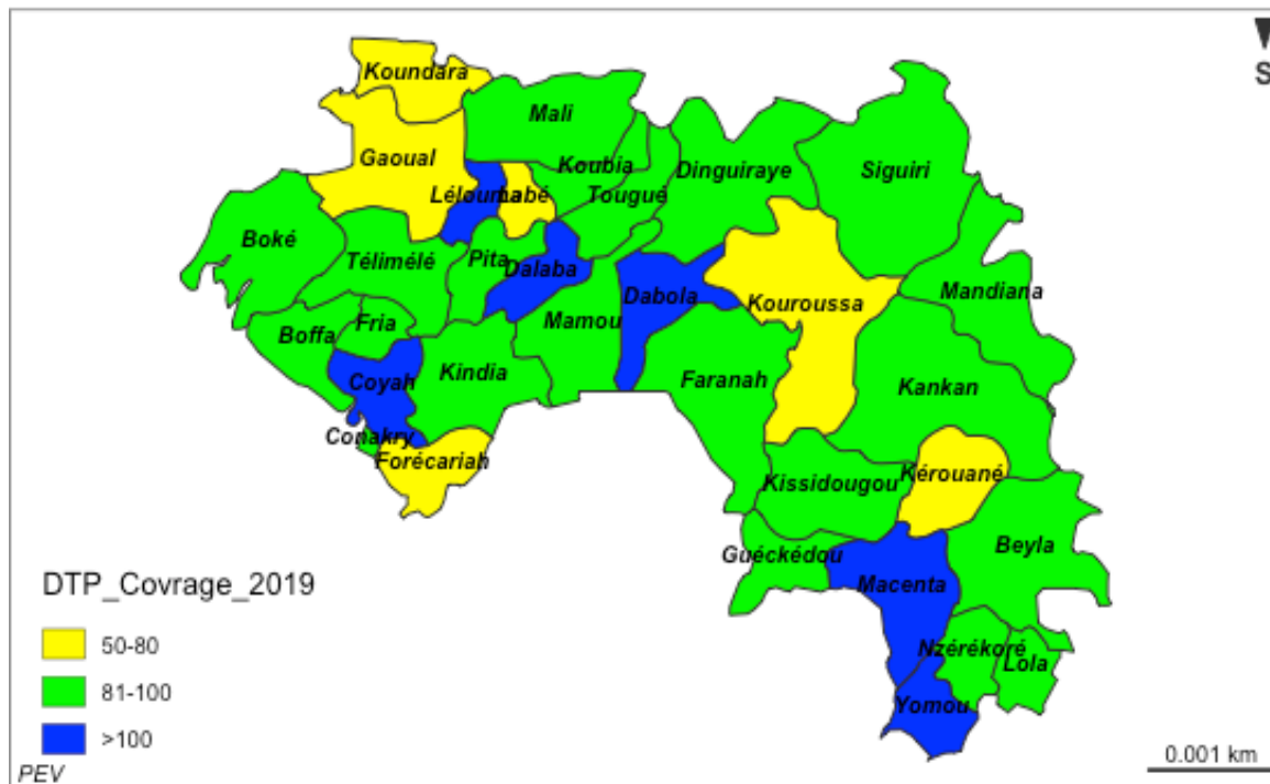
Map1. half-yearly coverage for DTP 3 antigen in 2019
