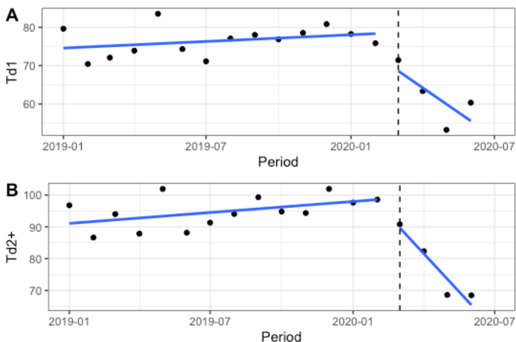
Figure 3. Trends in vaccine coverage of antigens (a) Td1 and (b) Td2
