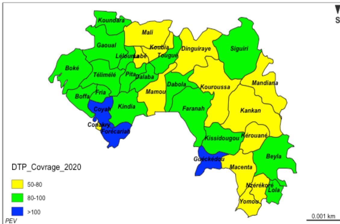
Map1. half-yearly coverage for DTP 3 antigen in 2020
