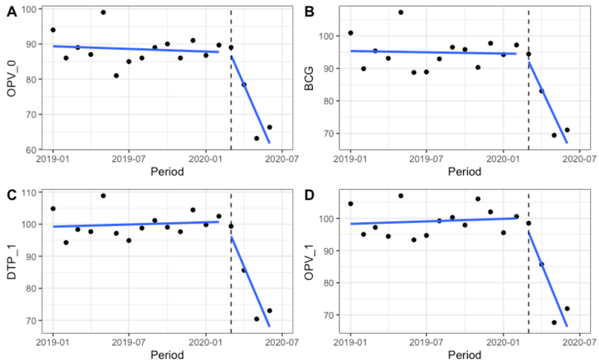
Figure 1. Trends in vaccine coverage for (a) OPV_0, (b) BCG, (c) DTP1, and (d) OPV1 antigens
