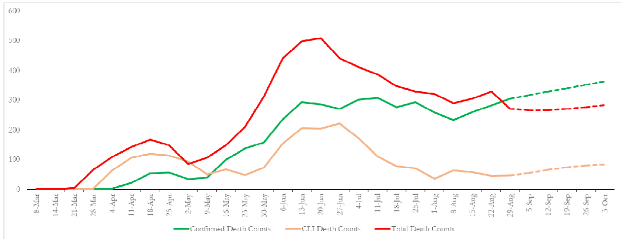
Figure 1: Actual and forecasted trends of confirmed, CLI, and total COVID-19 death counts in Bangladesh.
