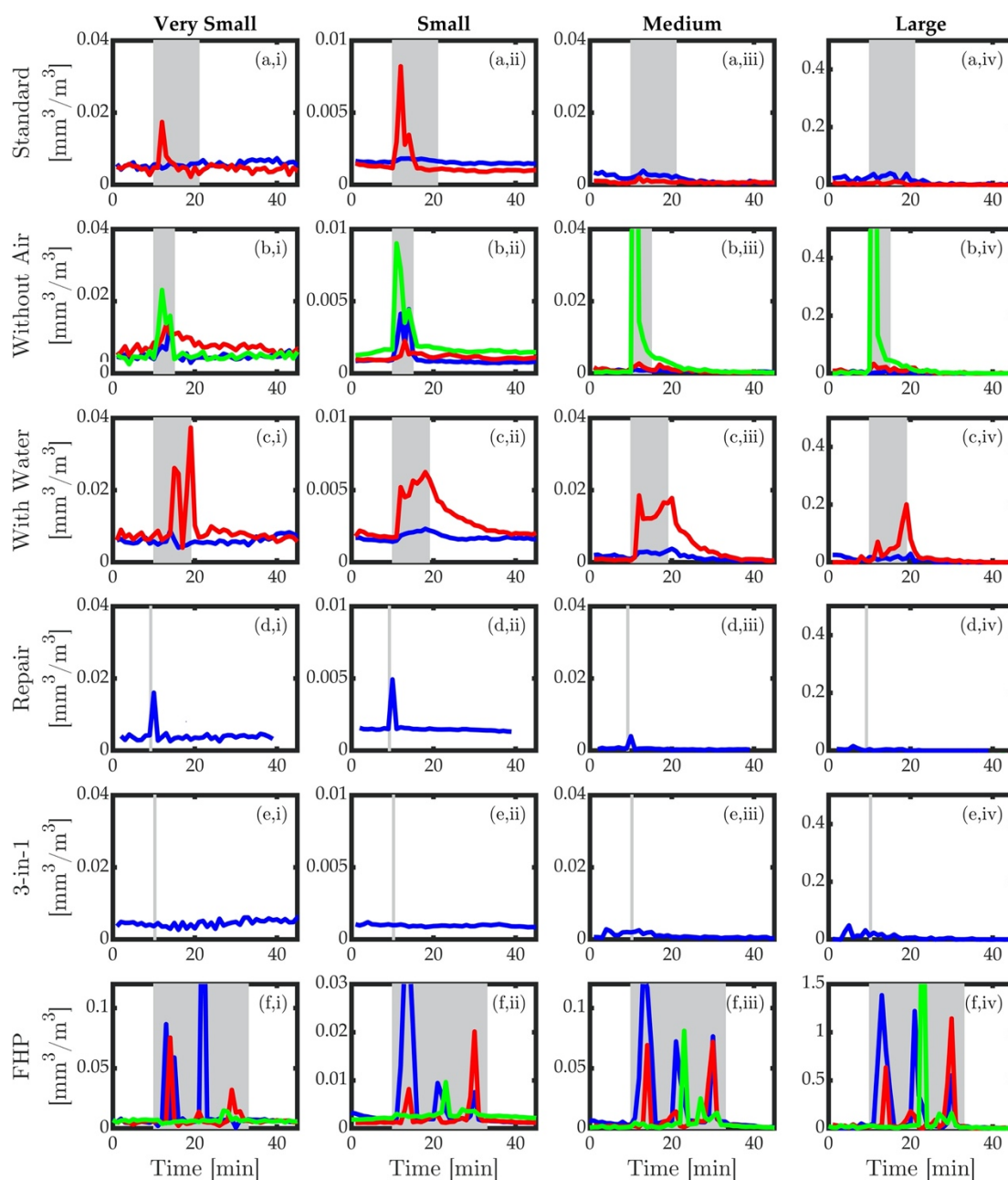
Figure 3. Variation in the measured concentrations of aerosols during each experiment. The rows correspond to the different procedures: standard debond (a), debond without air (b), debond with water (c), repair of two teeth using standard debond approach (with air only) (d), and 3-in-1 air water syringe (e) and debond using the fast-hand piece (f). The columns show the concentrations for various size ranges
