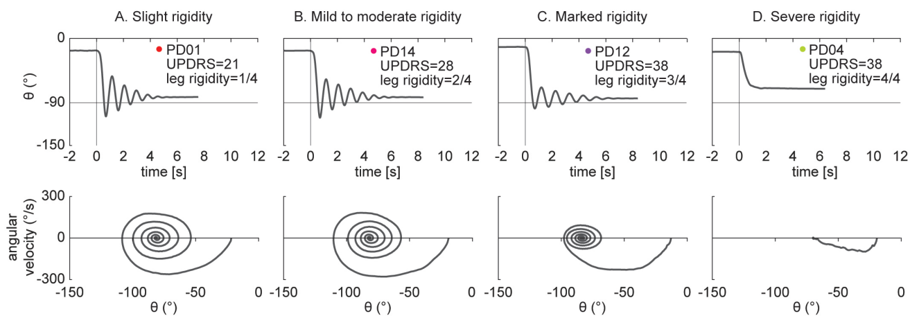
Figure 3. Example of pendulum test kinematic traces in four PD individuals with increasing levels of lower leg rigidity (as measured by following the UPDRS guidelines). Slight rigidity ( A ). Mild to moderate rigidity ( B ). Marked rigidity ( C ). Severe rigidity ( D ).
