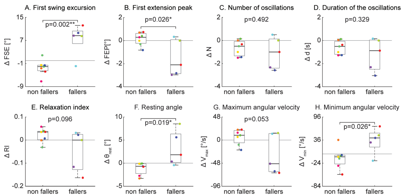
Figure 7. Variation of kinematic outcomes of the pendulum test during an activation maneuver in non-fallers and fallers. Asterisks denote significant values ( p < 0.05 ).
