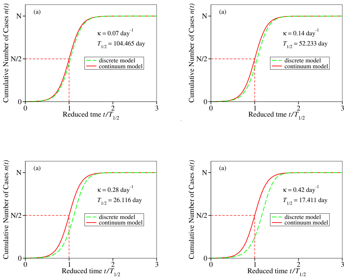
Figure 1: Cumulative number of infection cases described by means of logistic growth models employing continuous and (“exact”) discrete time representation (equations (4) and (2), respectively) for several typical values of the infection rate \kappa indicated in the inset. Time on the x -axis is expressed in units of the half-time T_{1/2} .
