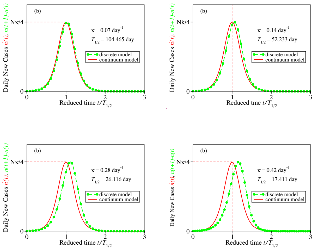
Figure 2: Epidemiological curves depicting daily numbers of new infections described by means of logistic growth models employing continuous and (“exact”) discrete time representation (equations (5) and 2), respectively) for several typical values of the infection rate \kappa indicated in the inset. Time on the x -axis is expressed in units of the half-time T_{1/2} .
