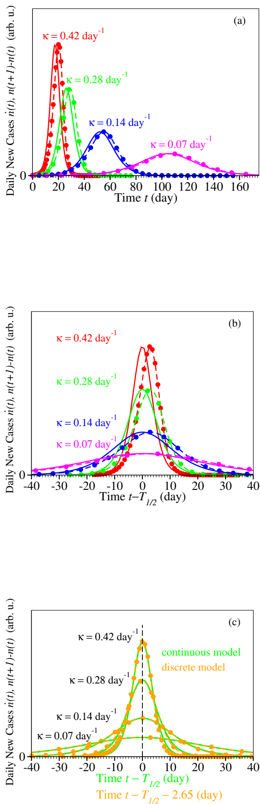
Figure 3: Epidemiological curve depicting daily numbers of new infections described by means of logistic growth models employing continuous and (“exact”) discrete time representation for several typical values of the infection rate \kappa indicated in the inset.
