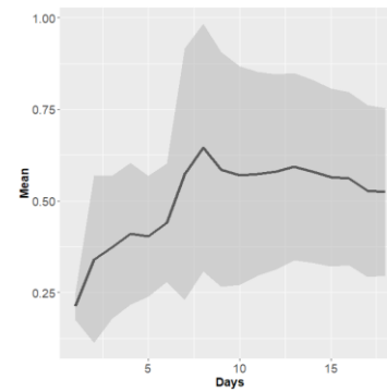
Fig. 4d. The Estimated Infectivity Rates
