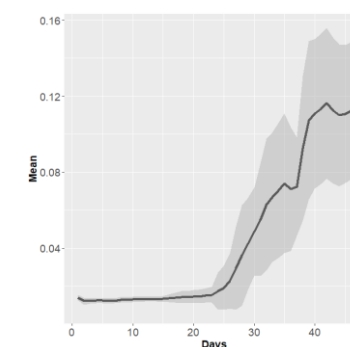
Fig. 3d. The Estimated Infectivity Rates
