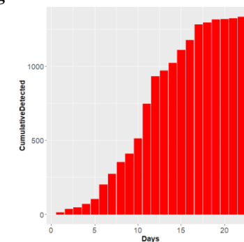
Fig. 4b. Total Confirmed Positive Cases
