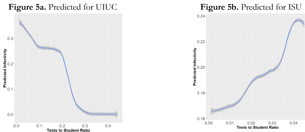
Figure 5. The Non-linear Curve Fitting Predictions for Infectivity with respect to the Testing Intensity
