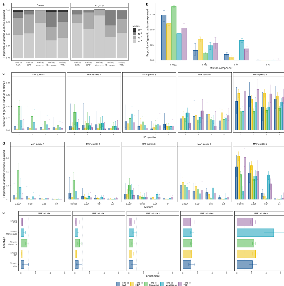
Figure 2. Genetic architecture for time-to-diagnosis of CAD, HBP, T2D and age-at-menarche and age-at-menopause, estimated using 2,975,268 markers and unrelated European ancestry individuals from the UK biobank. We ran BayesW models with and without partitioning the markers to groups. Groups were created by splitting them first to MAF quintiles and each MAF quintile was further split to quartiles based on LD giving us a total of 20 groups. (a) Mean proportions of genetic variances explained by each of the mixtures with the groups model and without groups model, groups model and no group model are yielding rather similar results; (b) distribution of proportion of genetic variance between mixtures for the model without groups, time-to-menarche stands out with almost all of genetic the variance attributed to the small mixtures; (c) distribution of proportion of genetic variance between LD quartiles within each MAF quintile, LD bins do not have a large impact on genetic variance partitioning as the credibility intervals are large and medians across LD quartiles are rather stable; (d) distribution of proportion of genetic variance between mixtures within each MAF quintile, mixture allocations tend to be similar compared to no groups model; (e) enrichment (ratio of proportion of genetic variance and proportion of markers attributed to each MAF quintile group) value for each phenotype, enrichment of higher than 1 represents that the markers are explaining more of the genetic variance compared to their count proportion and vice versa. (b)-(e) median and 95% credibility intervals are shown, (c)-(e) are group models. For all of the traits most of the genetic variance is coming from common SNPs (MAF quintile 5).
