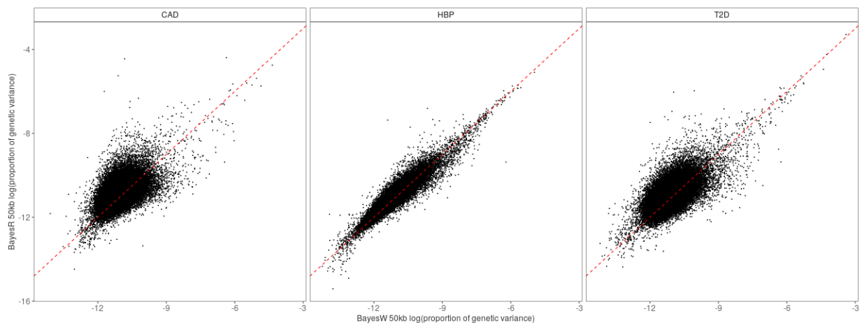
Figure S9. Logarithm of mean proportion of genetic variance explained by each 50kb region using either time-to-event model (BayesW groups) or case-control approach (BayesRR). Three analysed phenotypes were (time-to-)HBP, (time-to-)T2D and (time-to-)CAD and the analysis was conducted on unrelated UK biobank individuals. The BayesW groups model is using 20 MAF-LD groups and BayesR model is using 36 groups based on genomic annotations and MAF-LD binning. Both modelling framework reach similar conclusions in terms of discovered regions: for HBP, T2D and CAD the correlation between the logarithm of results are 0.941, 0.647 and 0.554 respectively.
