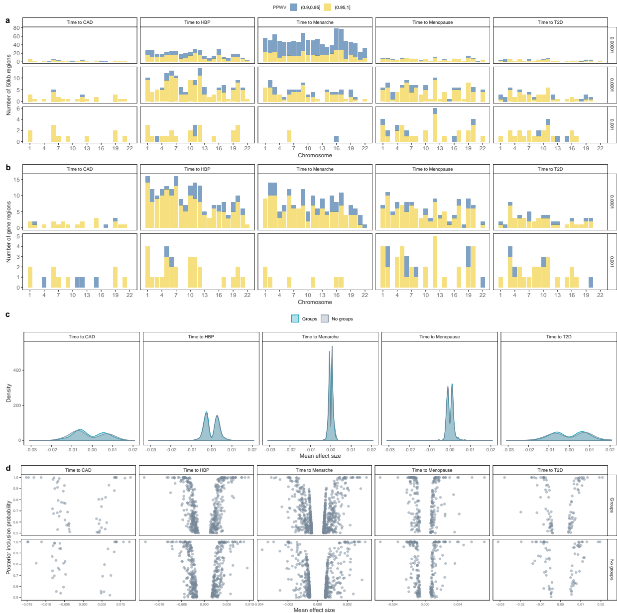
Figure 3. Regional and individual SNP contributions to the time-to-diagnosis of CAD, HBP, T2D and age-at-menarche and age-at-menopause. (a) Count of 50kb regions with high PPWV (Posterior Probability Window Variance). We split the genome into 50kb regions and then we calculated the probability that a region is explaining at least either 0.001%, 0.01% or 0.1% of the genetic variance (PPWV); (b) Count of gene-mapped regions with high PPWV. Each marker is mapped to a closest gene given that it is within \pm 50 kb from the marker, then for each of those gene-specific regions we calculate PPWV that the region explains either 0.01% or 0.1% of the genetic variance. Both (a) and (b) are using the groups model; (c) distribution of mean non-zero effect sizes for markers with posterior inclusion probability (PIP) > 0.5 for models with and without groups, we pick up mostly large effects for traits such as time-to-diagnosis of CAD or T2D whereas we find an abundance of small effects for age-at-menarche, we see a very small effect of penalisation in the case of group model; (d) relationship between mean non-zero effect size and posterior inclusion probability for markers with PIP > 0.5 with markers.
