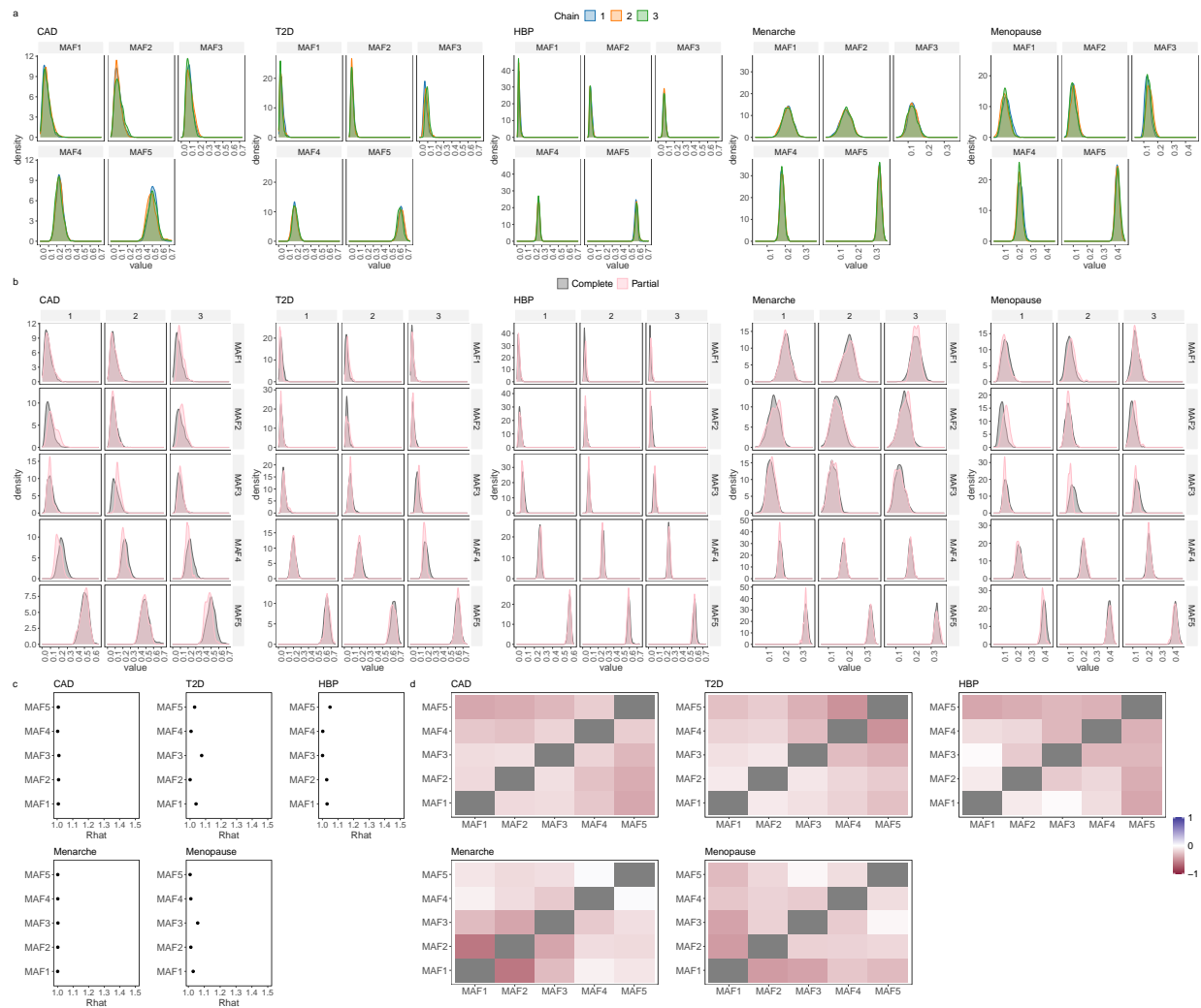
Figure S5. Convergence diagnostics of model chains for UK Biobank analysis with markers grouped into minor allele frequency (MAF) quintiles and then further subset into linkage disequilibrium (LD) quantiles. (a) overlapped density plots to compare the target distribution by chain showing each chain has converged in a similar space, for each MAF quintile and each trait. (b) overlapped density plots comparing the last 10 percent of the chain (green), with the whole chain (pink), showing that the initial and final parts of the chain are sampling the same target distribution for each MAF quintile and each trait. (c) the potential scale reduction factor comparing the among- and within-chain variance for each MAF quintile and each trait. (d) the cross-correlation between all parameters for each MAF quintile and each trait.
