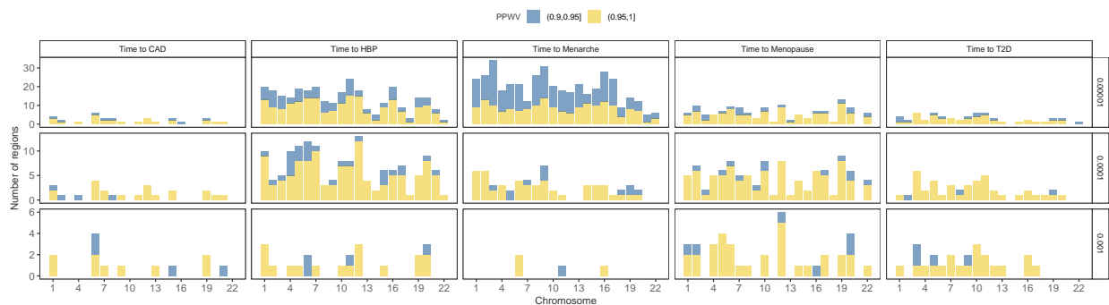
Figure S8. 50kb region contributions to the time-to-diagnosis of CAD, HBP, T2D and age-at-menarche and age-at-menopause using no groups model. Count of 50kb regions with high PPWV (Posterior Probability Window Variance). We split the genome into 50kb regions and then we calculated the probability that a region is explaining at least either 0.001%, 0.01% or 0.1% of the genetic variance (PPWV) using no groups model.
