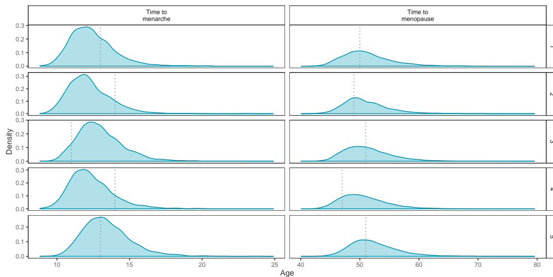
Figure S11. Posterior predictive distributions from BayesW for five random individuals from the Estonian biobank for time-to-menarche and time-to-menopause. BayesW enables calculating individual posterior predictive distributions, dotted lines indicate the true age at event. For age-at-menarche and age-at-menopause 94.8% and 92.3% of the true phenotypes from the Estonian biobank lie within 95% credibility intervals of those predictive distributions.
