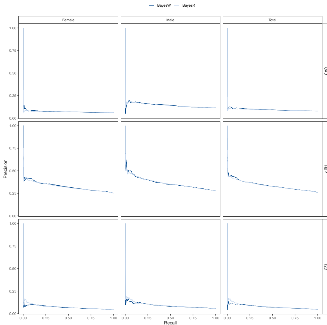
Figure S10. Precision-recall curves for predicting binary phenotypes (CAD, HBP, T2D) in Estonian biobank using either BayesR or BayesW model. Both models were trained on UK biobank data but BayesR model was using binary case-control phenotypes treating them as continuous variables and BayesW model was using respective time-to-diagnosis phenotypes. Precision-recall curves were drawn separately for females, males and all of the people (Total).
