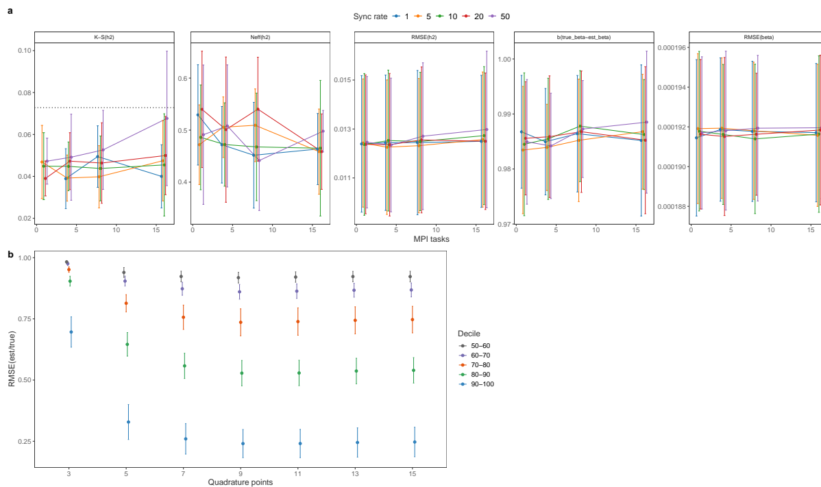
Figure S3. Computational recommendations for using BayesW. (a) Statistics to compare the MPI stability in various scenarios. Compared statistics: 1) Kolmogorov-Smirnov (K-S) test statistic for h^2 where every MPI setting was compared to the sequential version (one task, sync rate = 1), dotted line indicates the critical value for the K-S statistic at significance level of 0.01; 2) Number of effective samples per one iteration for h^2 after thinning of 5; 3) RMSE for h^2 ; 4) Linear regression slope when regressing the true marker values on the estimated ones; 5) RMSE for \beta parameters. We took the chromosome 1 of the UK biobank data set that was pruned for LD of 0.9 ( M = 230, 227 ), with randomly sampled N = 25, 000 individuals to make it similar to the real data setting. Phenotypes were simulated from Weibull distribution with heritability h^2 = 0.5 and the number of causal loci was p = 2, 500 . The models were run with three variance components (0.0001, 0.001, 0.01) with 10 simulations and 5 chains per MPI setting. The settings with 8 MPI tasks ( \sim 30, 000 markers per task) corresponds roughly to the setting in which full data sets are analysed. In the case where we are using very high synchronisation rate and split markers between many tasks, the estimates might deviate away from the sequential sampling results but for most settings updating markers synchronously will yield similar results compared to sequential sampling. (B) Impact of the number of quadrature points on the estimation of effect sizes. Non-zero effect sizes were grouped to deciles and then RMSE(estimated/true) was calculated within each decile. We see that using more quadrature points makes the estimation better but it the improvement plateaus at some point.
