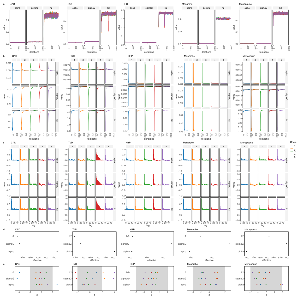
Figure S6. Convergence diagnostics of model chains for UK Biobank analysis with single marker group. (a) traceplot of the residual variance calculated as \pi^2/(6\alpha^2) labelled alpha, phenotypic variance attributable to SNP markers ( \sigma_{\text{G}} ), and the SNP-heritability ( h^2 ) of each trait, with colours representing the different chains. (b) a time series of the running mean of each chain, for each trait showing all chains approach the same mean value for each parameter. (c) lagged autocorrelation plot of each chain, for each trait and (d) effective number of uncorrelated sampled obtained for each trait. As phenotypic variance is being partitioned it is not expected that posterior estimates obtained are entirely uncorrelated. (e) Geweke z-score statistic comparing the initial part of the chain to the final part, for each trait.
