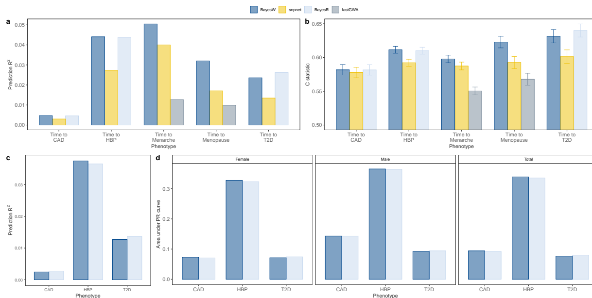
Figure 4. Prediction into the Estonian biobank. BayesW and snpnet methods were used for all of the phenotypes; BayesR was used to see how case-control model predicts time-to-diagnosis phenotypes (CAD, HBP, T2D); fastGWA was used to see how marginal model performs when predicting continuous traits. (a) Prediction R^2 when predicting Estonian martingale residuals of time-to-event phenotypes using either BayesW, snpnet, BayesR or fastGWA model trained on the UK biobank data, martingale residuals were calculated from Cox PH model with an intercept and sex if applicable; (b) Harrell's C-statistic with 95% confidence intervals, calculated from Cox PH model where true phenotype was regressed on the genomic prediction and gender data (for CAD, HBP and T2D); (c) Prediction R^2 when predicting Estonian binary phenotypes (CAD, HBP, T2D) using either model based on time-to-event data (BayesW) or case-control data (BayesR), the binary phenotypes that were used for the comparison were adjusted for age and sex; (d) Area under Precision-recall curve when predicting Estonian binary phenotypes (CAD, HBP, T2D) using either BayesW or BayesR, areas under curve were calculated separately for females, males and everyone combined.
