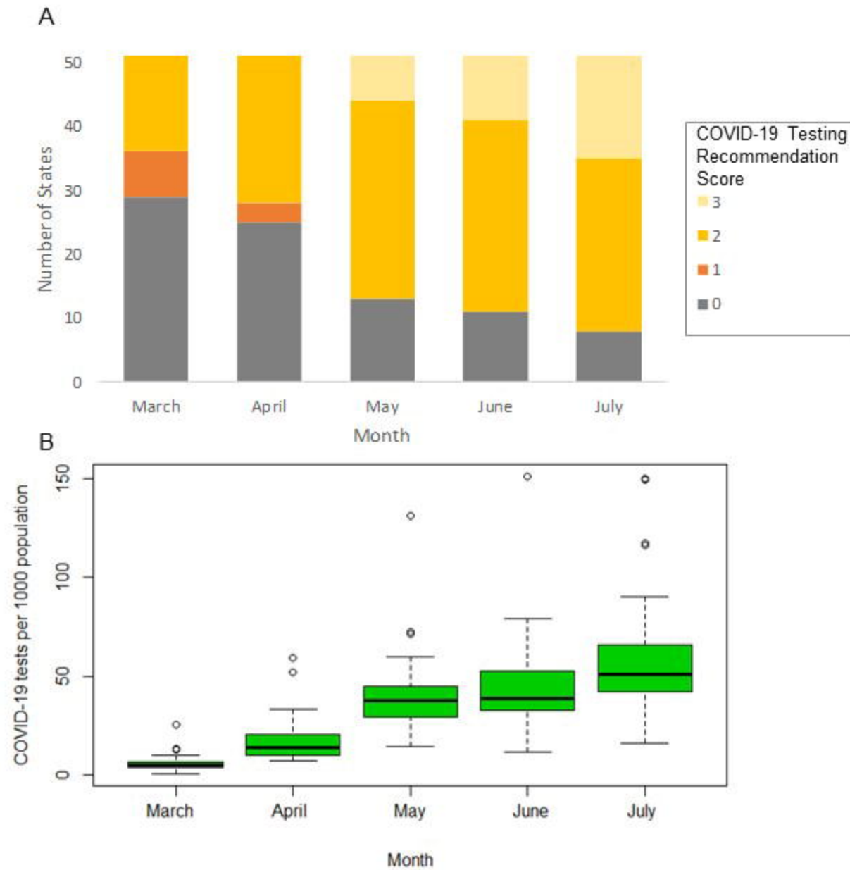
Figure 3. COVID-19 testing recommendation scores (A) and COVID-19 tests per 1000 people (B) from March-July, 2020 in the United States
