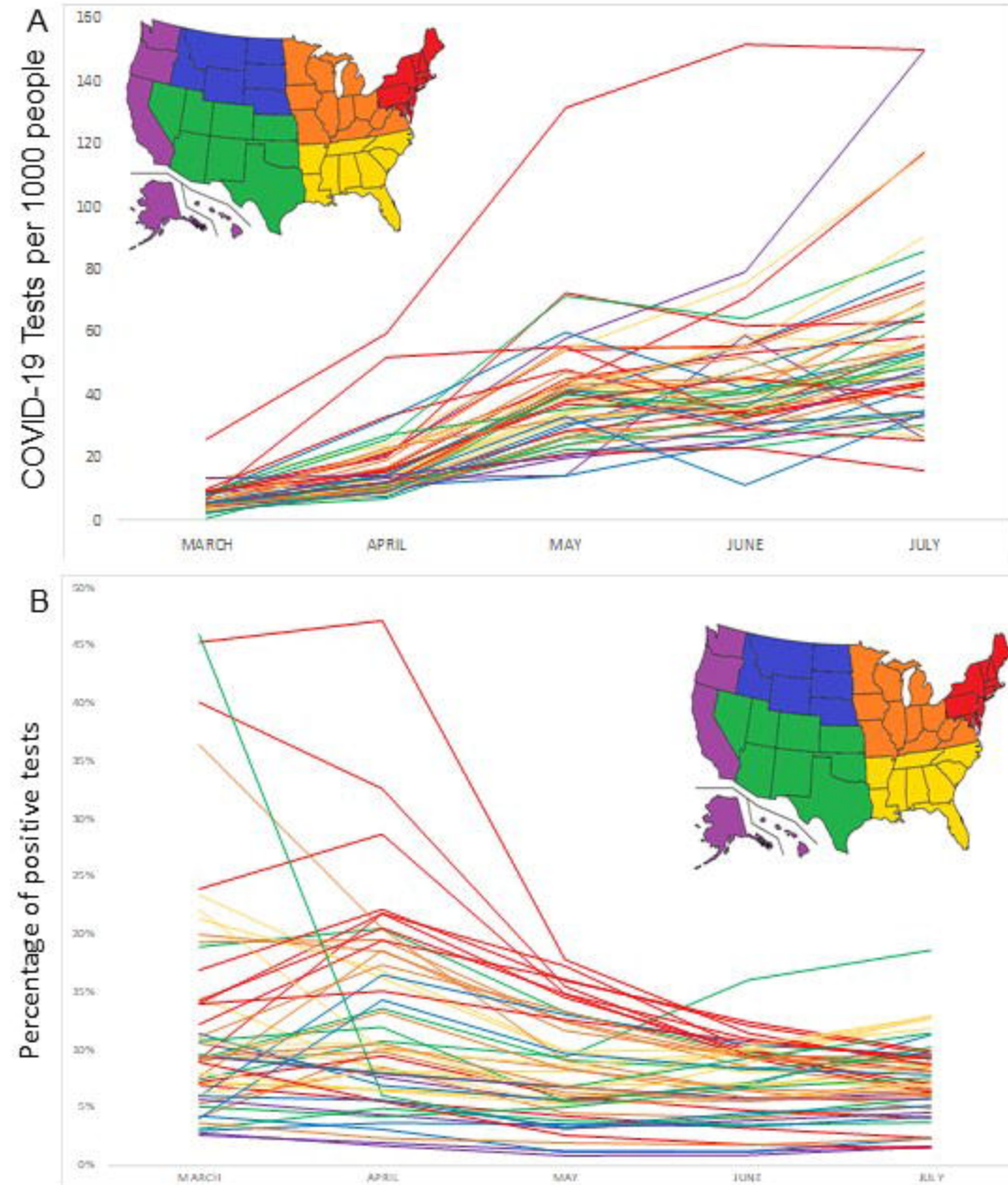
Figure 2. COVID-19 tests per 1000 population in the United States (A), and the percentage of positive COVID-19 tests (B), March-July 2020. Each state has a line; colors of lines are determined by geographic region per the inserted map.
