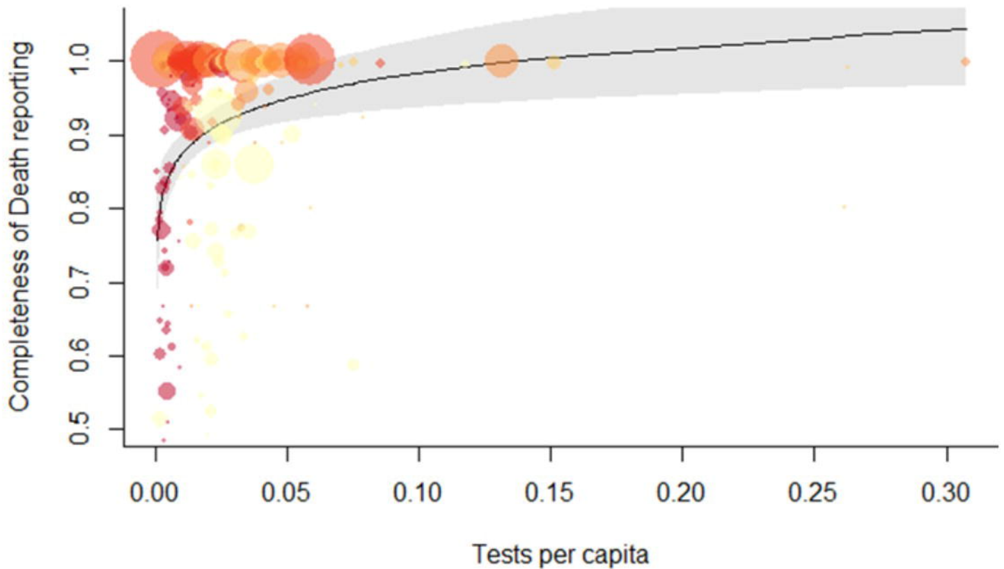
Figure 4. Association between the rate of testing for SARS-CoV-2 ( per capita ) and the completeness of death reporting, as measured by the ratio between reported COVID-19 deaths and excess deaths due to pneumonia/influenza/coronavirus (PIC). The line +/- 95% confidence intervals represents the trend as estimated from a generalized additive model. The size of the circles is proportional to the number of excess deaths due to PIC in each state. The color depicts the month (March-July)—earlier months are darker colors, later months are lighter.
