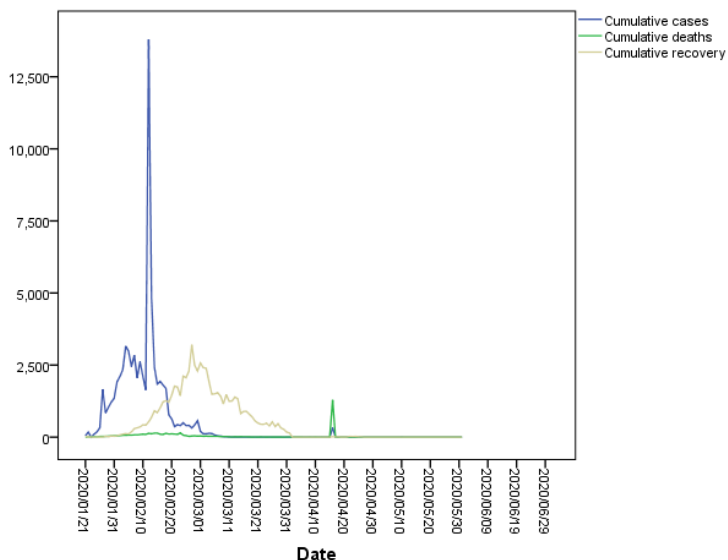
115 Fig.3 First-order difference processing time series figure ( d=1 )
