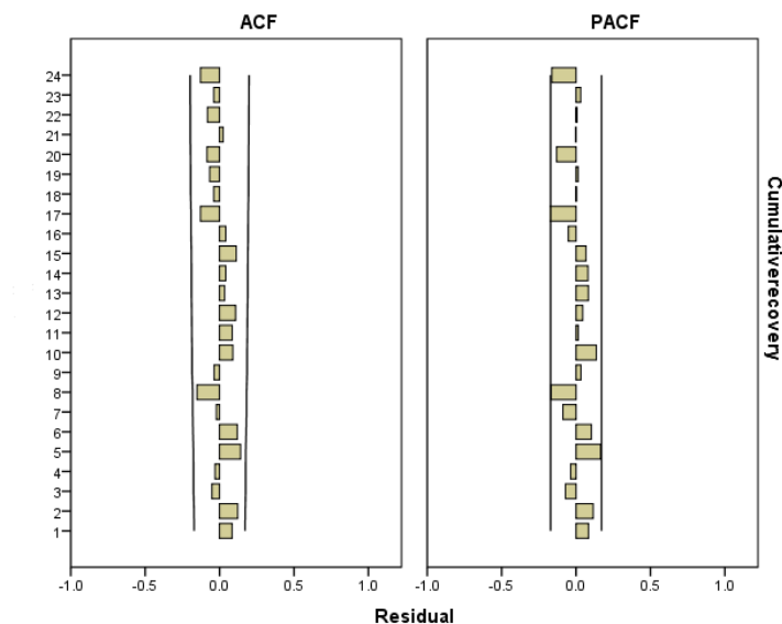
133 Fig.5 Residual sequence figure of ARIMA model for the cumulative cases, deaths, recovery in 134 Hubei Province
