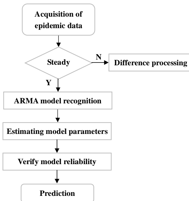
Fig.1 The flowchart of ARIMA model
