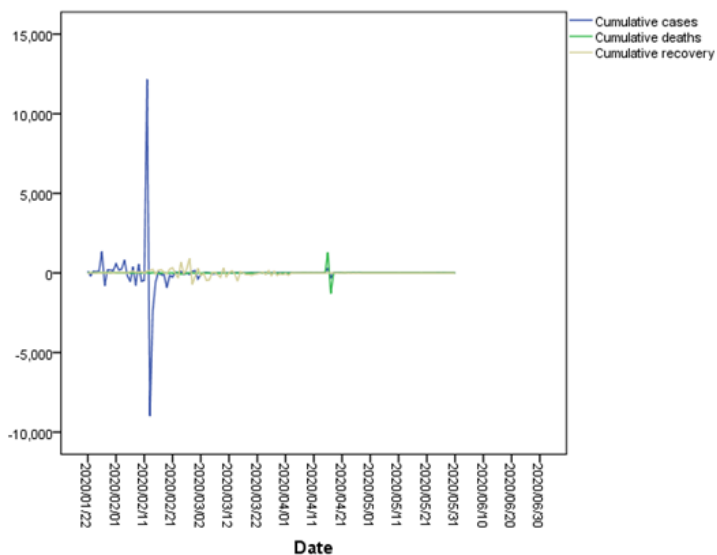
Fig.4 Second-order difference processing time series figure (d=2)
