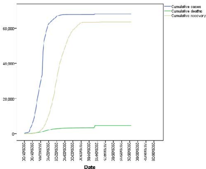
113 Fig.2 The cumulative cases, deaths, recovery original time series figure
