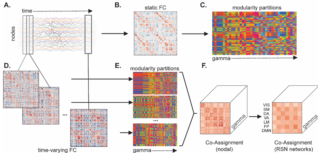
Figure 1. Network construction and modularity workflow. (A) Time series for all nodes were correlated to generate (B) a sFC matrix, on which modularity was performed to obtain (C) a set of partitions across the \gamma (gamma) parameter range. Sliding window was used to compute (D) tvFC matrices for partially overlapping time frames. (E) Modularity on each window generated a set community partitions, which were then used to compute (F) co-assignment over time at each \gamma . Pairwise nodal co-assignment values were then averaged with and between canonical resting state network (RSN) blocks. VIS: Visual; SM: Somatomotor; DA: Dorsal Attention; VA: Ventral Attention; LM: Limbic; FP: Frontoparietal; DMN: Default Mode Network.
