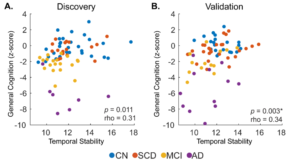
Figure 6. Relationship of general cognition and temporal stability of the ventral attention resting state network. Individual points represent individual participants from either the (A) Discovery or (B) Validation samples, colored by diagnostic group. CN: Cognitively Normal; SCD: Subjective Cognitive Decline; MCI: Mild Cognitive Impairment; AD: Alzheimer's disease. rho: Partial Spearman's rho (age, sex, and education adjusted). * denotes FDR-significant correlation in the Validation sample.
