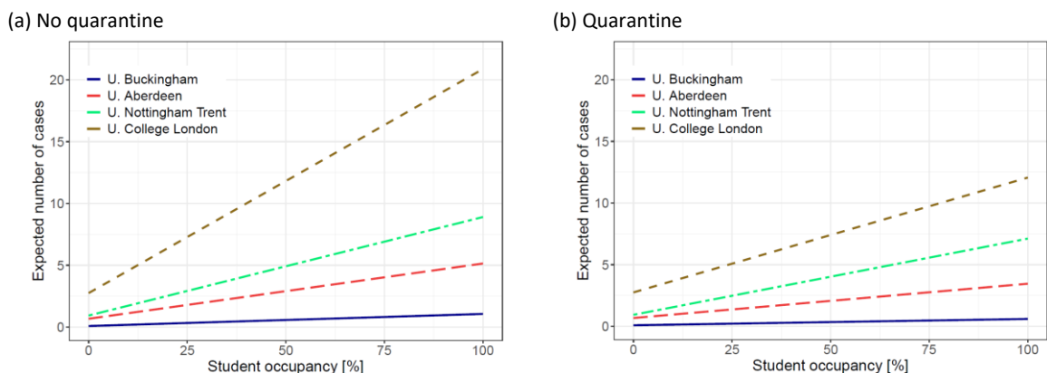
Figure 4. The expected number of cases arriving on campus as a function of student occupancy for selected HEIs assuming (a) no quarantine or (b) quarantine for international students outwith from travel corridors.
