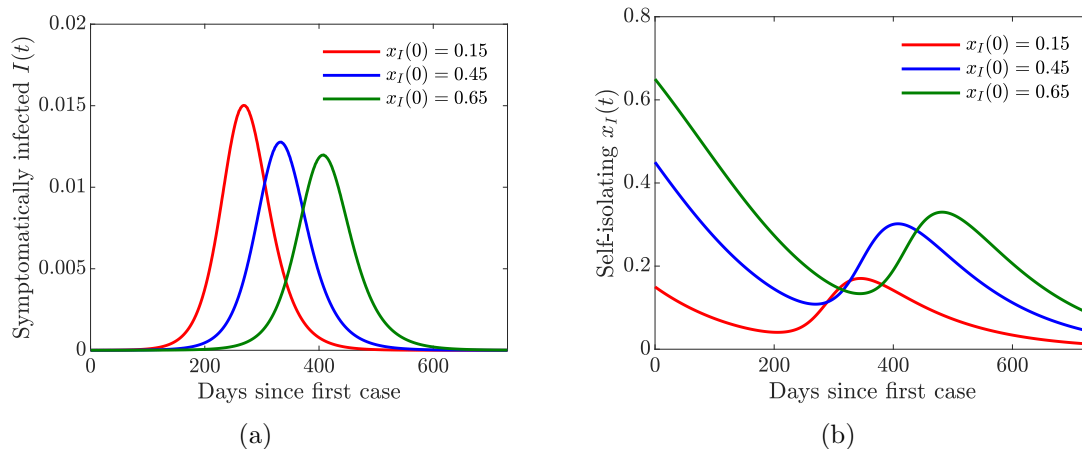
Figure 6: Simulations of the COVID-19 model with dynamic human behavior (15) with various initial proportions x_I(0) of symptomatically infected individuals willing to self-isolate. The social learning rate of infected individuals is \kappa_I = 100 , and the sensitivity to self-isolation is \varepsilon_I = 0.00008 . (a) The progression of the proportion of symptomatically infected individuals I(t) . (b) The progression of the proportion of symptomatically infected population willing to self-isolate.
