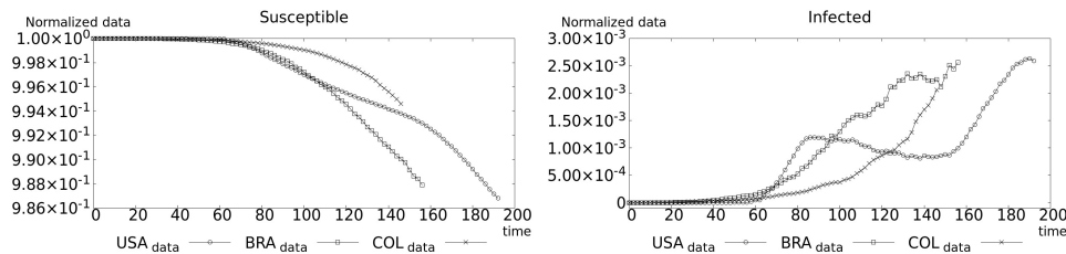
Figure 3: Susceptible (left), and infected (right) normalized data
