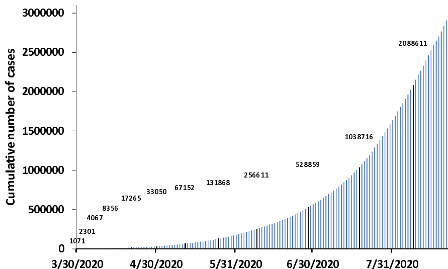
Figure 1. Doubling time of the cumulative cases
