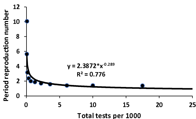
Figure 4. Regression fit for period reproduction number on tests per 1000 population
