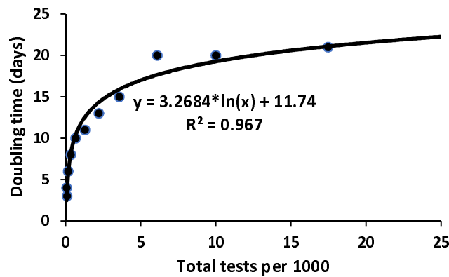
Figure 3. Regression fit of doubling time on tests per 1000 population
