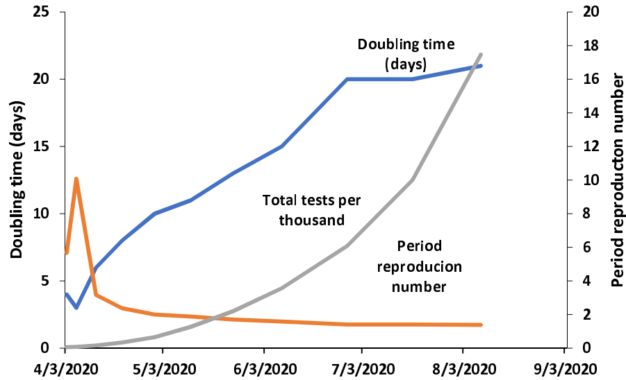
Figure 2. Trend of doubling time, tests, and period reproductive number
