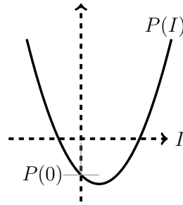
Figure 2: Graph of P(I) in the case when R_0 > 1 .
