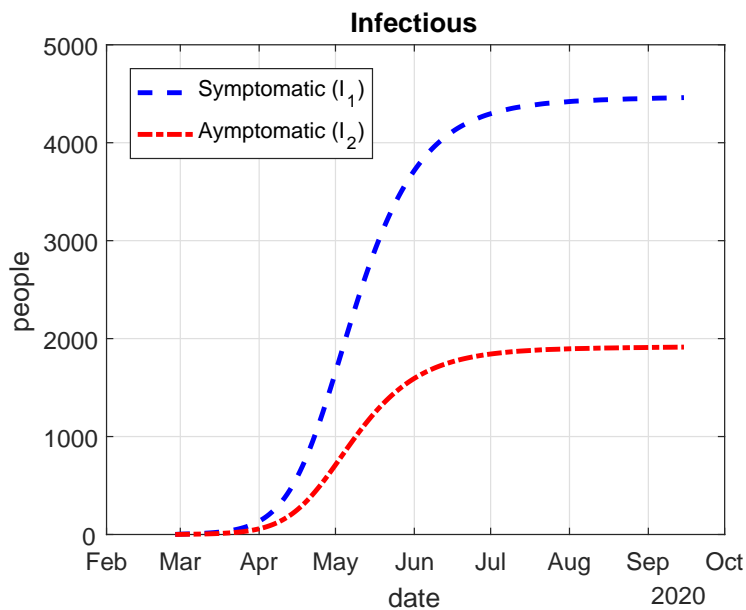
Figure 10: Number of symptomatic ( I_1(t) ) and asymptomatic ( I_2(t) ) infectious individuals estimated by the model.
