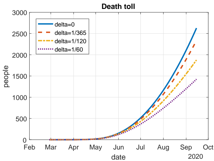
Figure 12: Death toll estimated by the model for different values of \delta .
