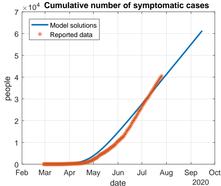
Figure 6: Cumulative number of symptomatic infectious individuals estimated by the model ( C(t) ) and reported data.
