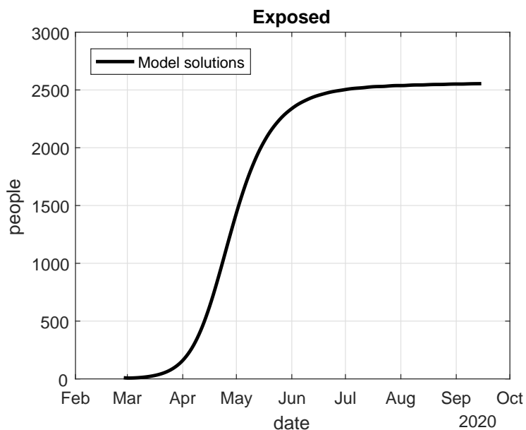
Figure 9: Number of exposed individuals estimated by the model ( E(t) ).
