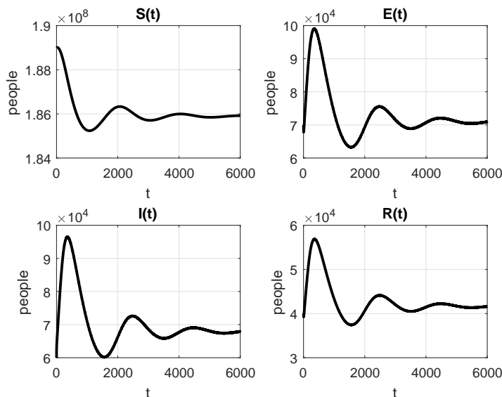
Figure 4: Time evolution of the solutions for the model when r = 0.08 and the endemic equilibrium is locally asymptotically stable.
