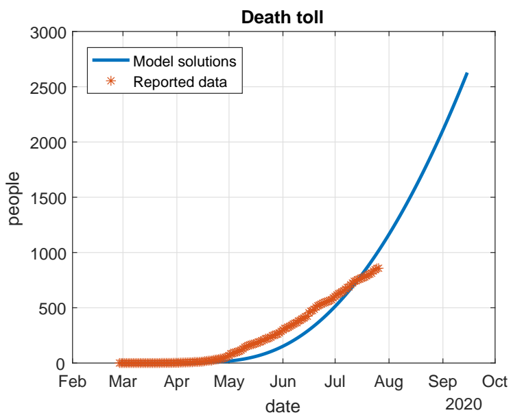
Figure 8: Death toll estimated by the model ( R_1(t) ) and reported data.
