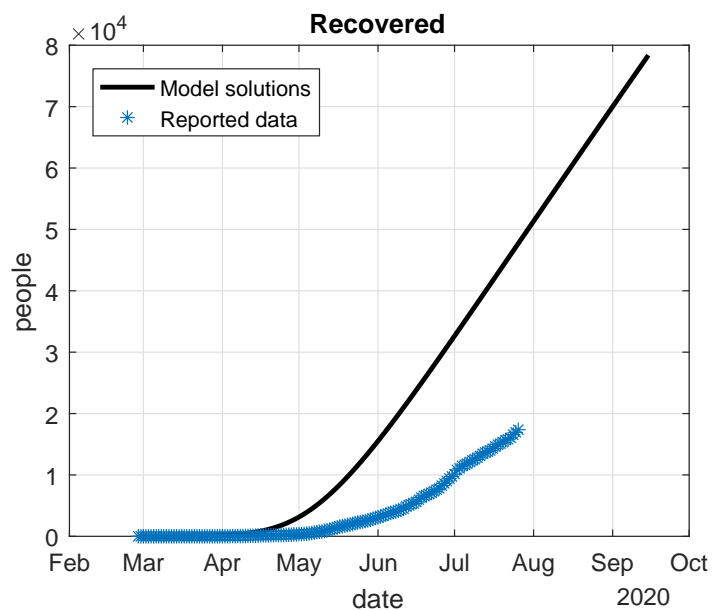
Figure 7: Number of recovered individuals estimated by the model ( R(t) ) and reported data.
