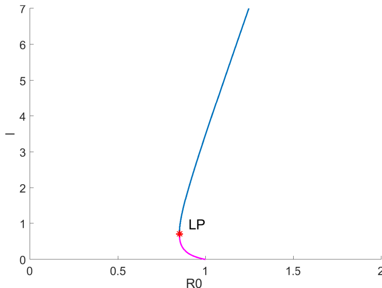
Figure 3: Backward bifurcation diagram of the model. The horizontal axis represents the value of the basic reproduction number. The vertical axis indicates the size of infected population at equilibria. LP denotes the saddle-node bifurcation point.
