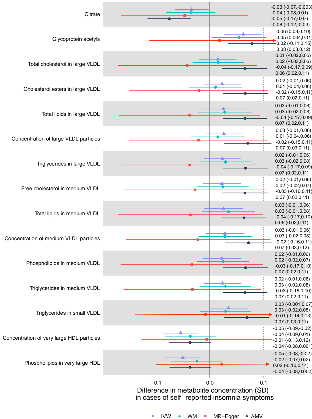
Figure 3: Mendelian randomization and age-, sex- and BMI-adjusted multivariable regression analyses results for select associations of insomnia symptoms with NMR-derived metabolomic measures.
