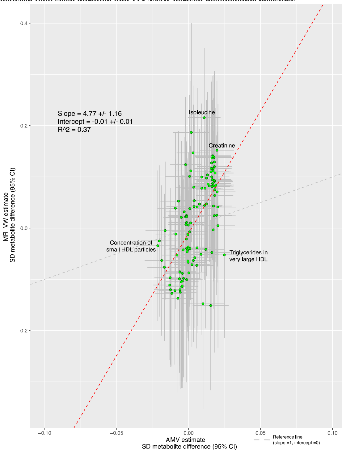
Figure 5: Comparison of the point estimates of the IVW Mendelian randomization and age-, sex- and BMI-adjusted multivariable regression analyses for the associations between total sleep duration and 112 NMR-derived metabolite measures
