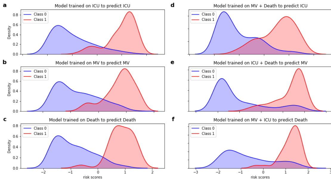
Fig. 2 - Density Plots. a-c. Density plots for single outcome models. d-f. Density plots for aggregate models predicting unspecific outcome.
