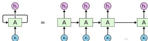
Fig. 2. The structure of recurrent neural networks
