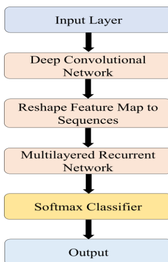
Fig. 3. The workflow of the CNN-RNN architecture for COVID-19 diagnosis
