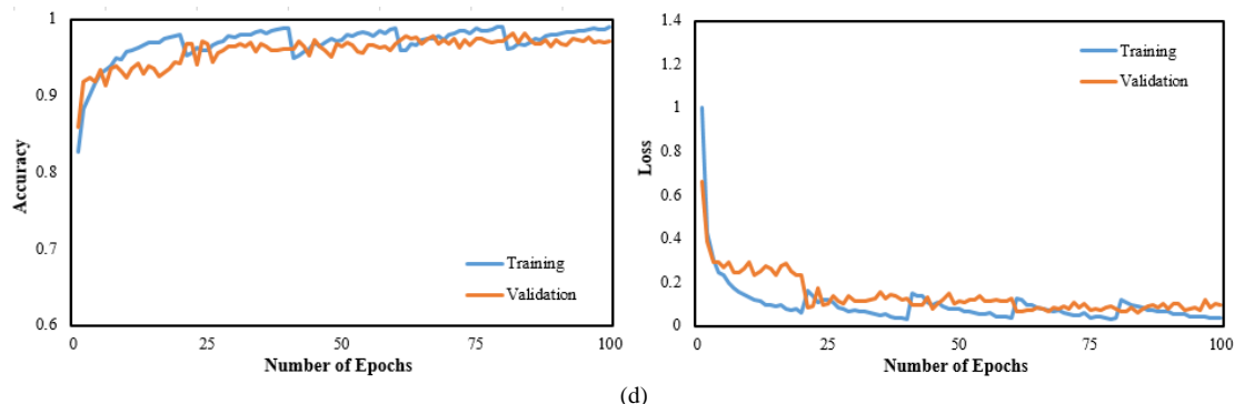
Fig. 5. Accuracy and loss curve of four CNN-RNN architectures. (a) VGG19 (b) DenseNet121(c) InceptionV3 (d) Inception-ResNetV2
