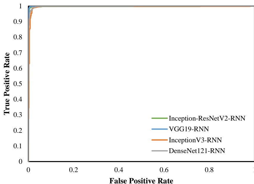
Fig. 7. ROC curves of four combined CNN-RNN networks
