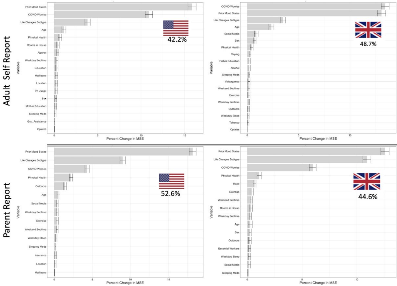
Figure 2: Variable importance and overall performance of Random Forest models predicting Current Mood States in the US and UK in both Adult self-report and parent report data. Variables are ranked by importance as measured by out-of-bag change in mean squared error (MSE), and those with a 95% lower bound above zero are shown here. Variables included: Prior Mood States, Life Changes Subtype, COVID Worries, physical health, age, sex, outdoors, exercise, social media, TV, videogame, weekend bedtime, weekend sleep, weekday bedtime, weekday sleep, insurance, rooms in house, government assistance, number in household, essential worker in household, Marijuana, Alcohol, vaping, opiates, sleeping medication and other drug use.
