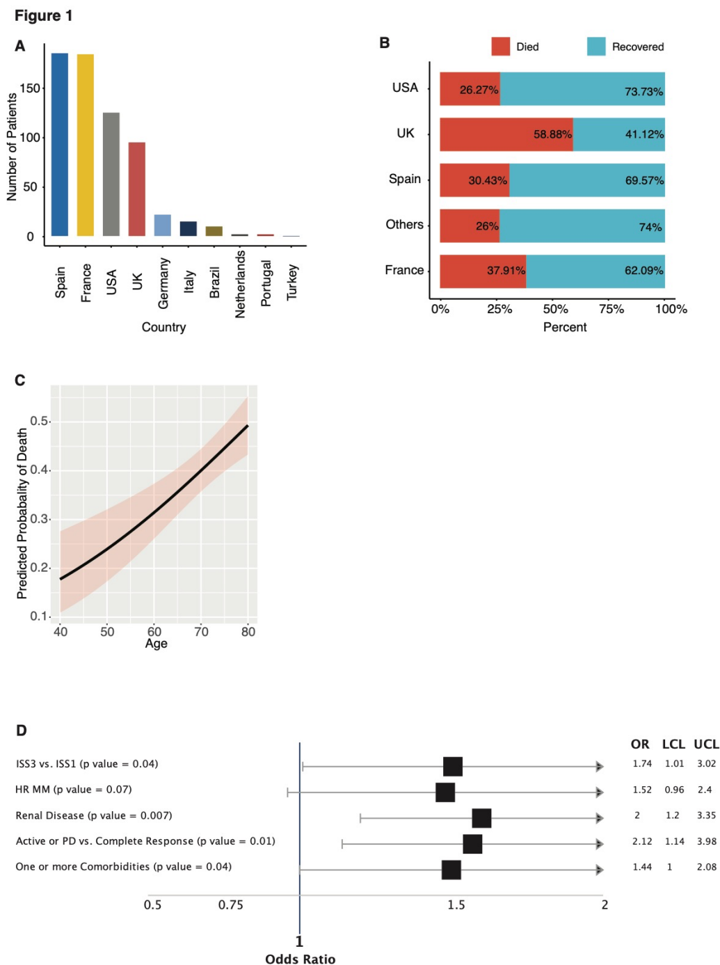
Figure 1: A) Number of patients in the IMS COVID-19 dataset with plasma cell disorders. B) Overall (outpatient and hospitalized) COVID-19 death rates in the dataset by contributing countries. C) Predicted COVID-19 outcome for MM patients by age. D) A forest plot for risk factors for MM patients from univariate analysis (OR, odds ratio; UCL, upper confidence level and LCL, lower confidence level).
