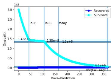
(a) Survivors and Just Recovered Populations: \phi = .03/10 * 10^{-8} * 0.5
