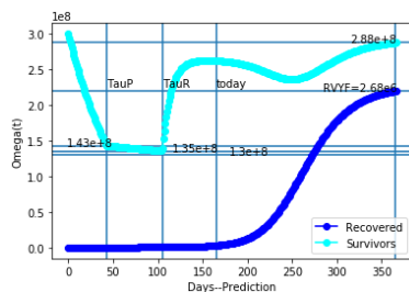
(a) Survivors and Just Recovered Populations: \phi = .03 * 10^{-8} * 0.5
