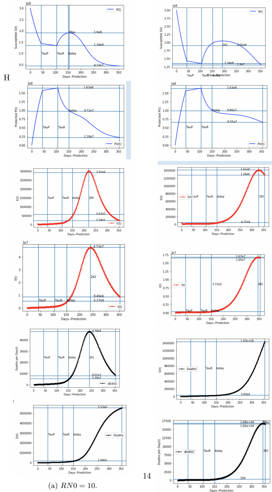
Figure 7: S, P, E, I, D, \dot{D} With Both Interventions RN0 = 10, 5
