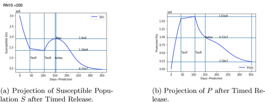
Figure 4: Projection of Susceptible and Protected Populations S and P .
