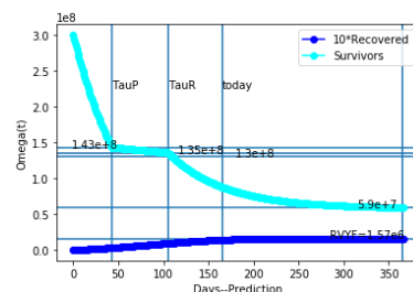
(b) Survivors and Just Recovered Populations: \phi = .03/10 * 10^{-8}
