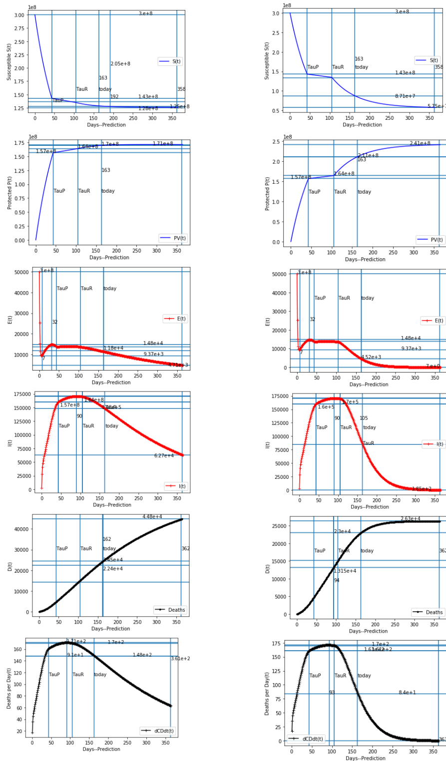
(a) S, P, E, I, D , and \dot{D} : \phi = .03/10 * 0.5
