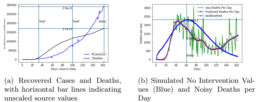
Figure 1: Views of Input Data
