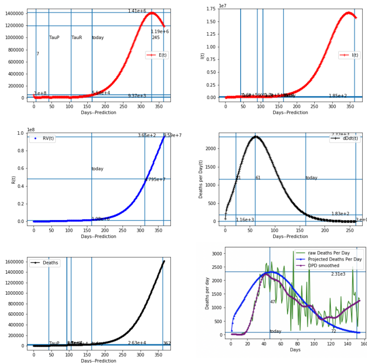
(a) Exposed, Recovered and Deceased Populations I, R, and D . (b) Infected, Recovered and Deceased Populations I, \dot{D} and \dot{D}_{SG}
