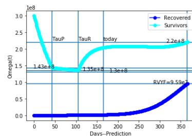
(b) Survivors and Just Recovered Populations: \phi = .03 * 10^{-8}
