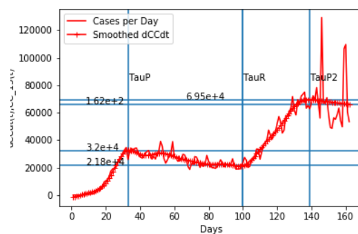
Figure 2: Noisy and Smoothed Cases per day Data showing the 3 Phases induced by the "Interventions" at t = \tau_P and t = \tau_R .
