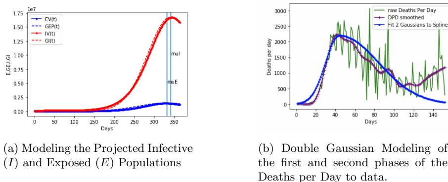
Figure 5: Examples of Gaussian Modeling.
