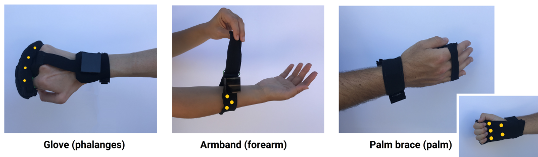
Fig. 2. Three stimulation devices used in the study. Each device contains 5 actuators of each type. Yellow dots are added to this figure to indicate actuator locations; not all actuators are visible here.
