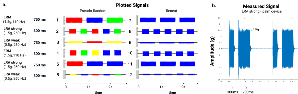
Fig. 3. a. 2.7 second plot of each stimulus (signals are 30 seconds long in total). Numbers 1-12 are used to refer to each signal. Changing colors indicate changing stimulus location in the pseudo-random patterns. b. Example accelerometer measurement of LRA actuator when embedded into the palm device.
