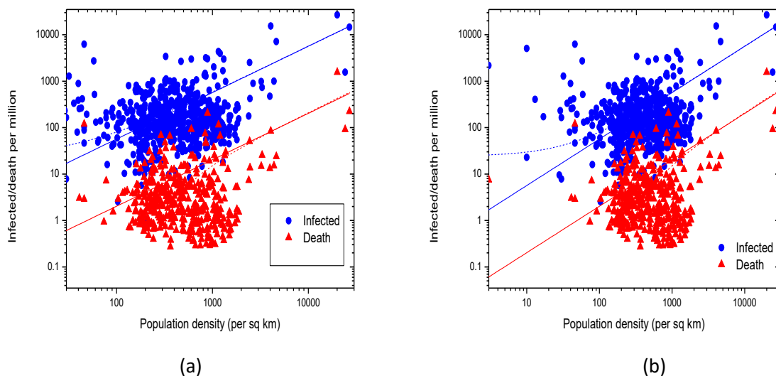
Figure 2: Same as Figure 1 but for the whole India, (a) up to 10 th September 2020 (b) till 5 th July 2020. The solid and dash lines describe the linear fit of the data with zero and non-zero intercepts respectively.
