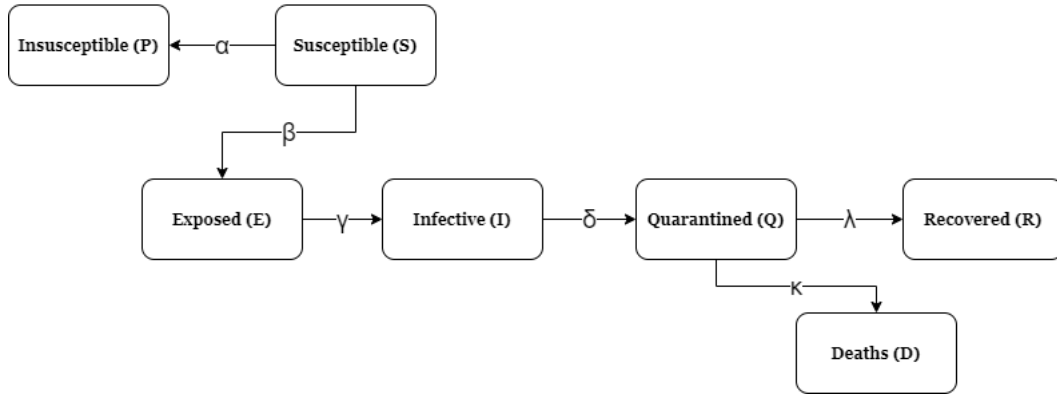
Figure 1: The interactions between the 7 compartments of the generalized SEIR model
