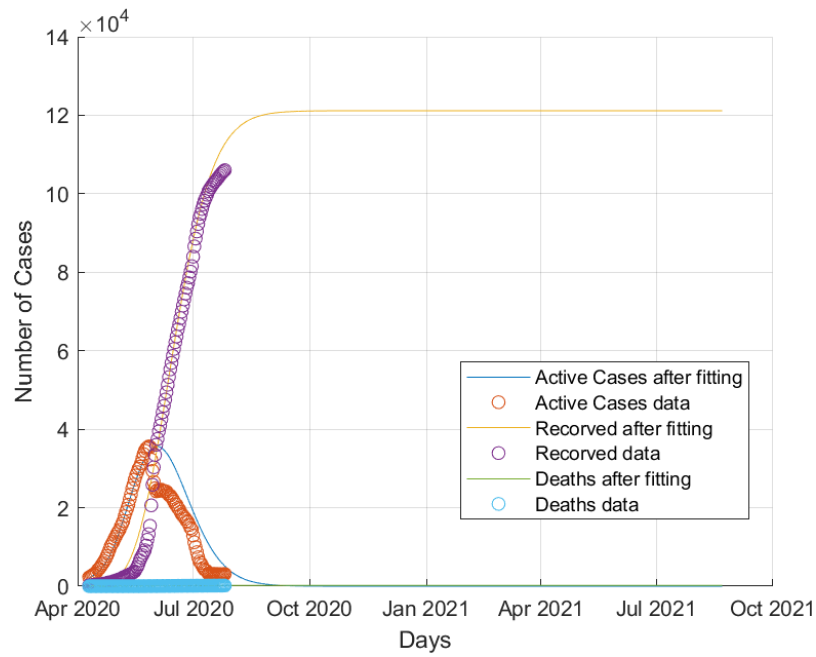
Figure 9: Collective behaviour of COVID-19 dynamics in Qatar.
