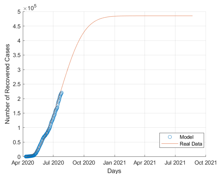
Figure 11: Recovered COVID-19 cases in Saudi Arabia.
