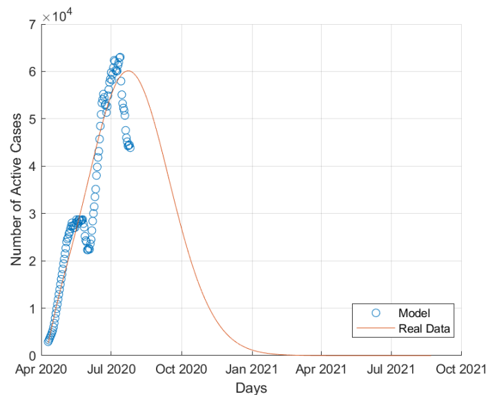
Figure 10: Active COVID-19 cases in Saudi Arabia.
