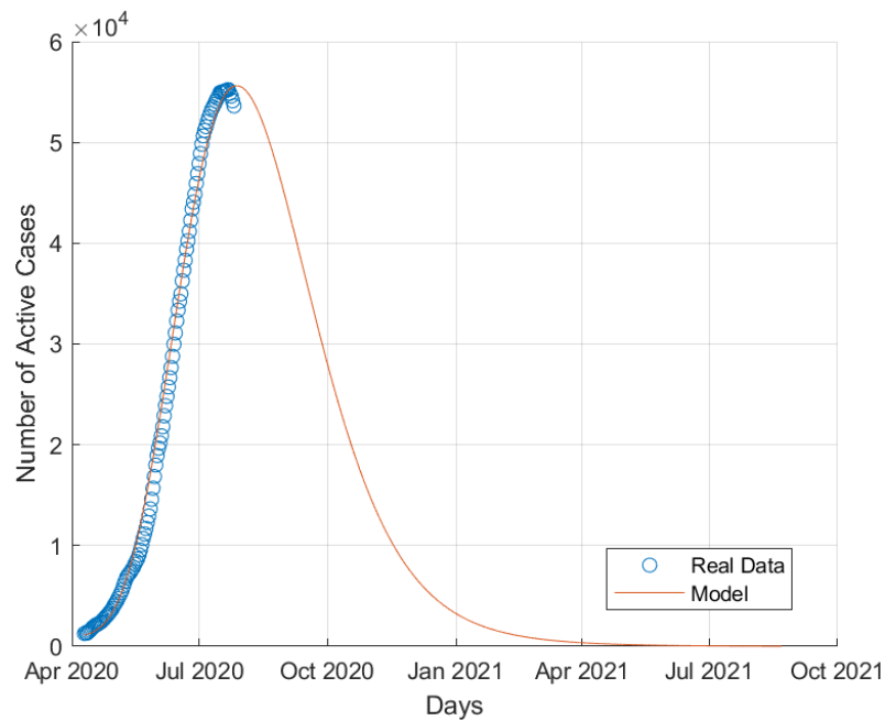
Figure 2: Active COVID-19 cases in Egypt.
