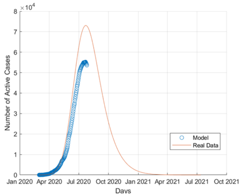
Figure 14: Egypt's active COVID-19 cases with pre-lockdown data incorporated
