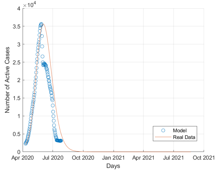
Figure 6: Active COVID-19 cases in Qatar.
