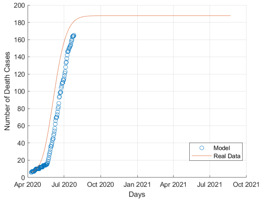
Figure 8: Death COVID-19 cases in Qatar.
