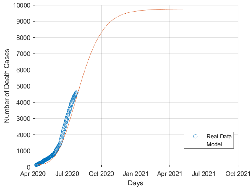
Figure 4: Death COVID-19 cases in Egypt.
