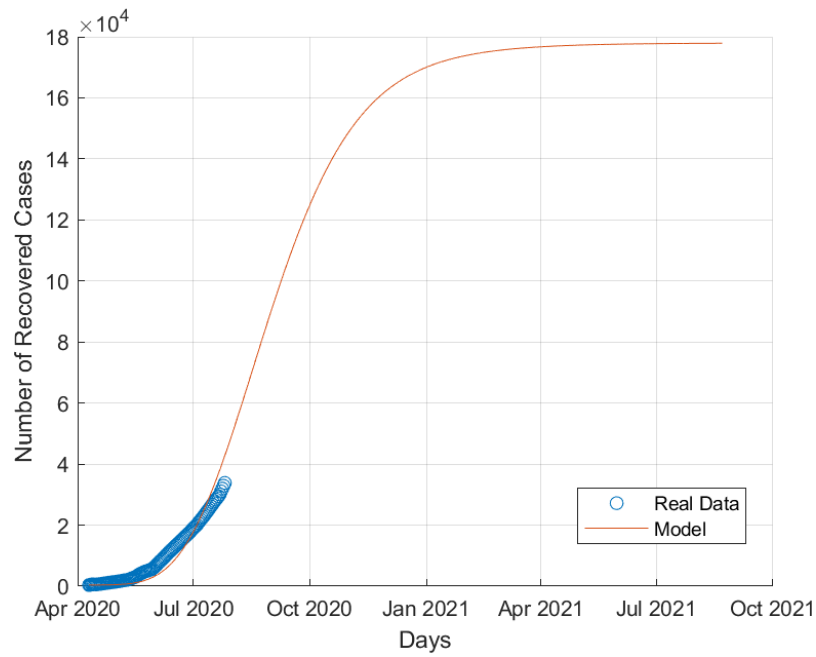
Figure 3: Recovered COVID-19 cases in Egypt.
