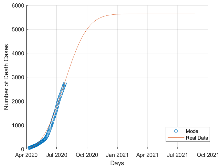
Figure 12: Death COVID-19 cases in Saudi Arabia.
