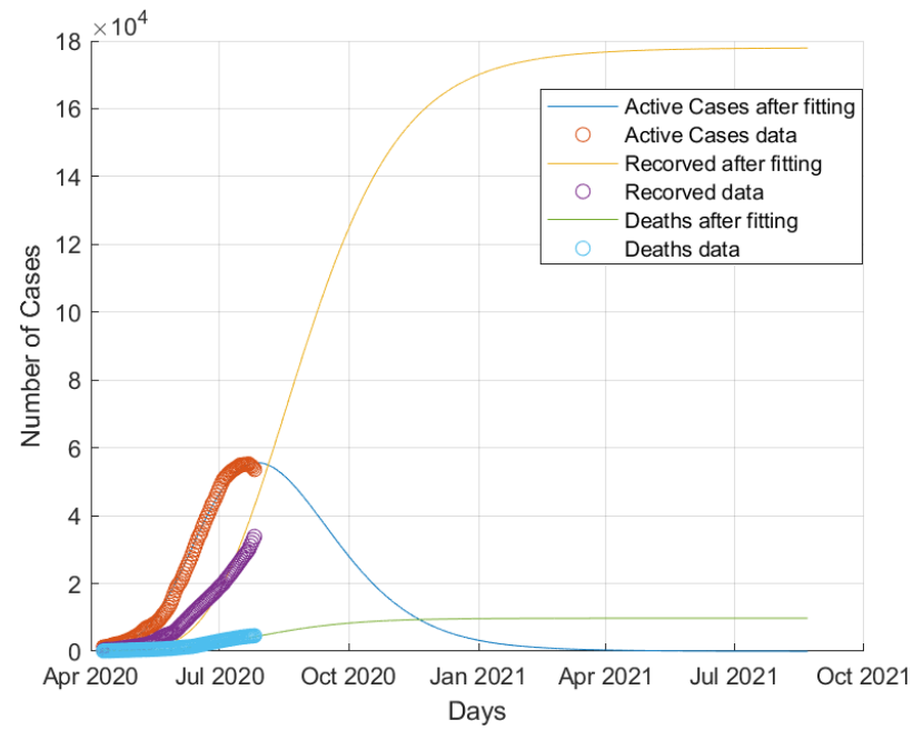
Figure 5: Collective behaviour of COVID-19 dynamics in Egypt.
