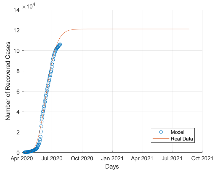
Figure 7: Recovered COVID-19 cases in Qatar.
