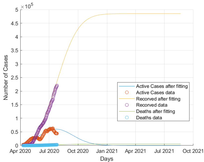
Figure 13: Collective behaviour of COVID-19 dynamics in Saudi Arabia.
