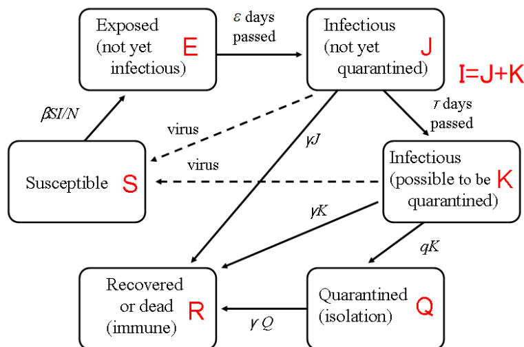
Figure 1: Flow chart of a delayed SEIQR model.
