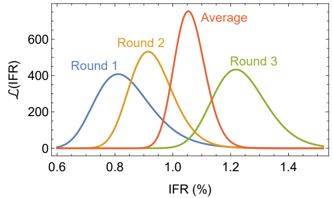
Figure 3. IFR likelihoods for Brazil for each of the 3 rounds and all rounds combined. Notice that round 3 exhibits a considerably higher IFR, which could be related to hospital bed saturation.
