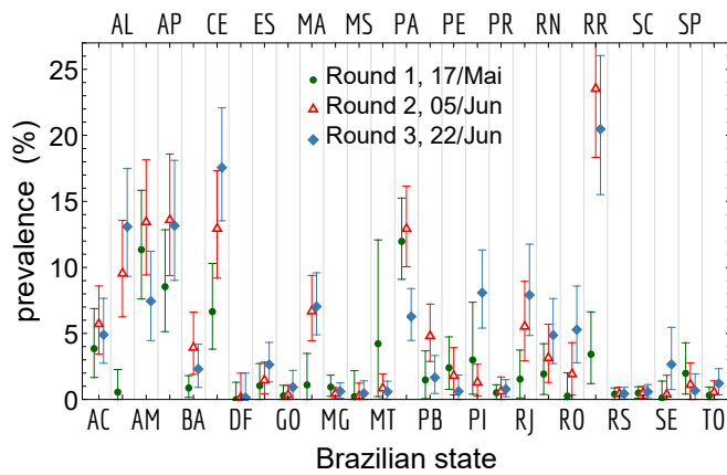
Figure 2. Prevalence (maximum likelihood and 95% CI) of COVID-19 antibodies in each of the 27 Brazilian states in the 3 rounds of the EPICOV19-BR survey.
