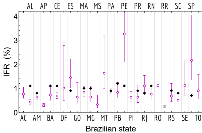
Figure 4. Combined IFR using all 3 rounds (maximum likelihood and 95%CI). The black dots represent model-based results by the Imperial College COVID-19 Response Team. 16 The horizontal red line is the IFR estimate for Brazil given in Table I. Two states have unreliable combined IFR results and are shown in light gray: PA has a significant decrease in p_a in round 3 that cannot be a simple fluctuation; RR has a very low IFR in round 2 which is in tension with the other rounds and artificially shrinks the CI.
