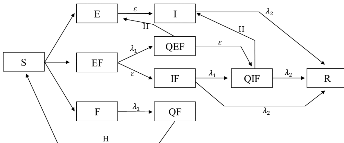
Figure 1: Model Flowchart. Here, all ten possible states of an agent in the model are depicted. In addition, parameters of \lambda_1 shows the rate at which agents self-isolate due to fear, and parameter \lambda_2 shows the rate at which disease infected agents recover from the disease. Parameter H shows the rate at which agents finish their self-isolation and return to circulation.
