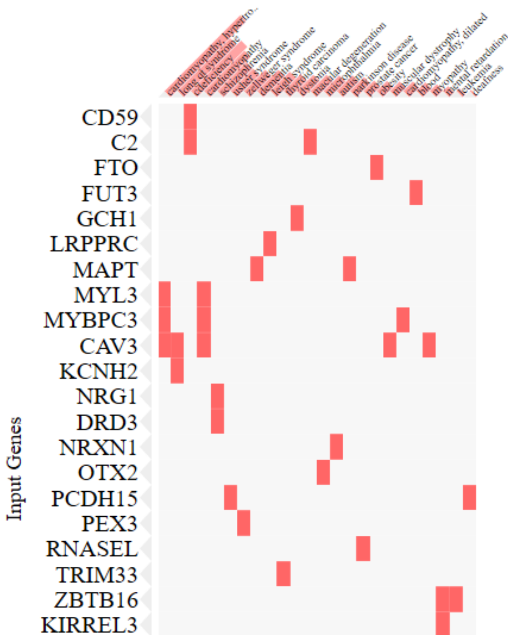
Figure 1. Enrichment of MIM terms with associated genes in the chronotype-linked genes. Enrichr was used to calculate enrichment using Fisher's exact test. The MIM terms on the top x axis are organized by order of enrichment p value (Supplemental Table 2). Gene names underlying enrichment are shown in the clustergram.
