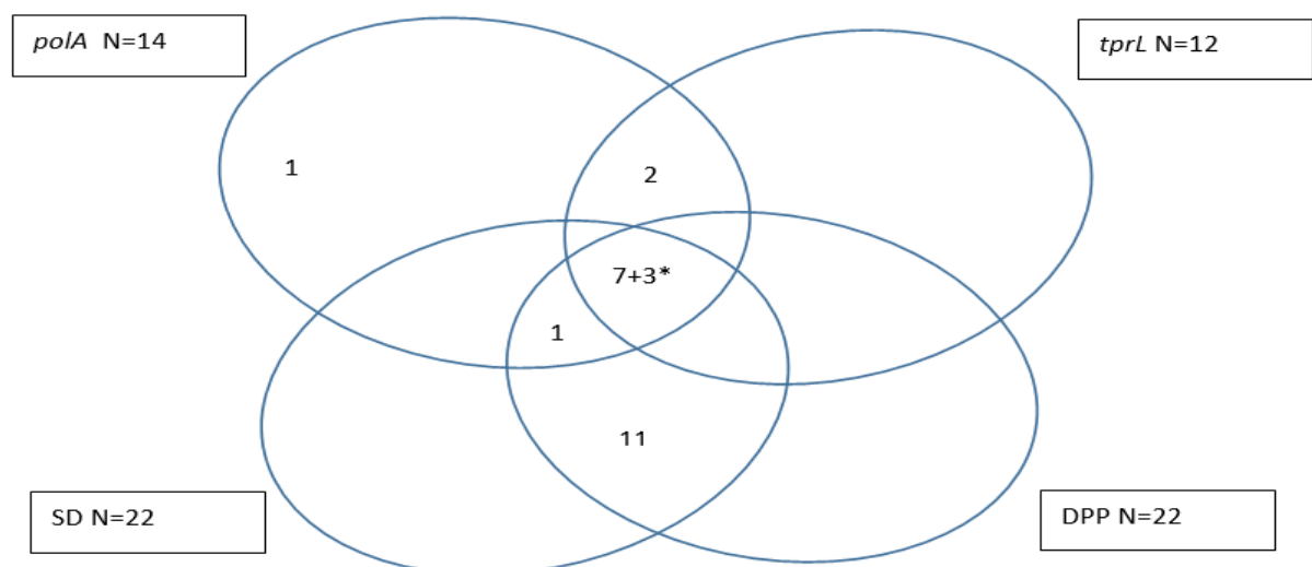
Fig 2. Number of samples with positive assay results in polA qPCR, tprL PCR , SD, and DPP.
