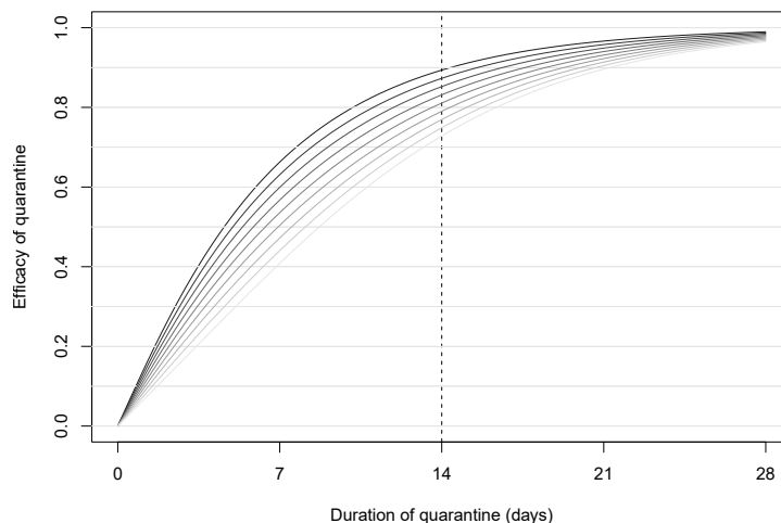
Figure 7: Probability c that the quarantine is successful as a function of its duration t_q . From dark to light grey: fraction \pi of asymptomatic or undetected cases varying from 0.1 to 0.9 by steps of 0.1.
