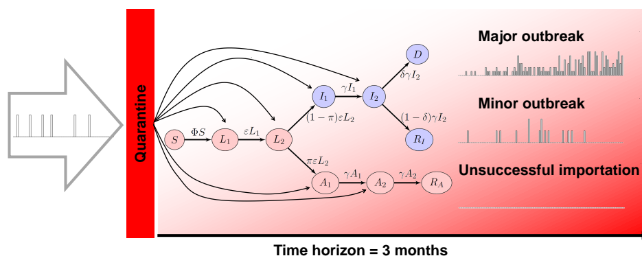
Figure 3: Input-output setting: imports arrive through transport, are potentially funnelled through quarantine, then enter one of the infected compartments. The three types of outcomes considered are shown on the right.
