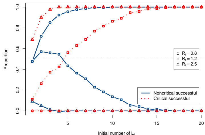
Figure 4: Proportions of critical (dotted red) and noncritical successful (solid blue) importations as a function of the initial number of imported L_1 cases. Circles: \mathcal{R}_t = 0.8 , squares: 1.2 and triangles: 2.5.
