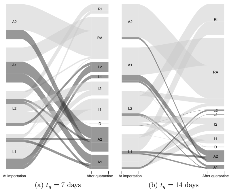
Figure 6: Evolution of the status of import cases during a (left) one or (right) two week quarantine period imposed upon arrival. Dark grey flows are individuals who are still a risk to the jurisdiction at the end of the quarantine period. Here, simulations were run for 2,500 individuals of each type of undetected cases L_1 , L_2 , A_1 , and A_2 entering quarantine.
