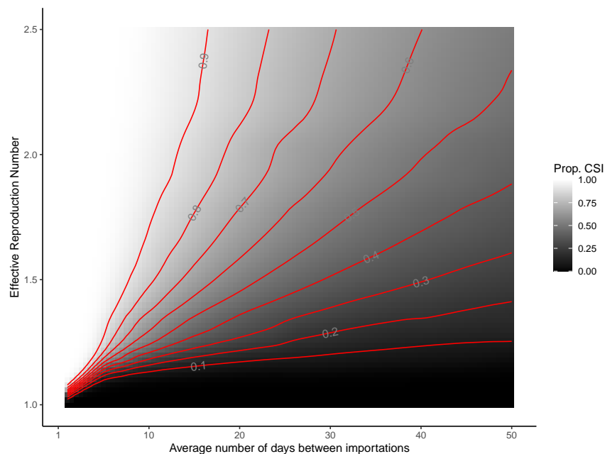
Figure ES.10: Proportion of critical successful importations (CSI) in a 3 month period for different values of the average number of days between two importations and \mathcal{R}_t , an indicator of NPI efficacy.
