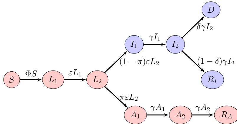
Figure ES.8: Flow diagram of the SL_1L_2I_1I_2A_1A_2R_I R_A D model. \Phi = \beta(I_1 + I_2 + \xi(A_1 + A_2) + \eta L_2) is the force of infection. Blue compartments are observable, with I_1 and I_2 usually indistinguishable and observed as I_1 + I_2 .
