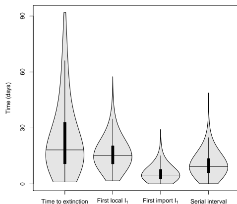
Figure ES.9: Time to extinction of the disease, first detected locally infected individual, first detected imported case, and serial interval. Base case simulation with S(0) = 142,906 (population of Prince Edward Island), L_1(0) = 1 and all other states equal to 0. Horizontal lines indicate the median value. Black rectangles are the inter-quartile range. Here, \mathcal{R}_t = 0.8 .
