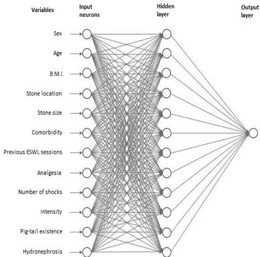
Fig.1: ANN nodes & connections
