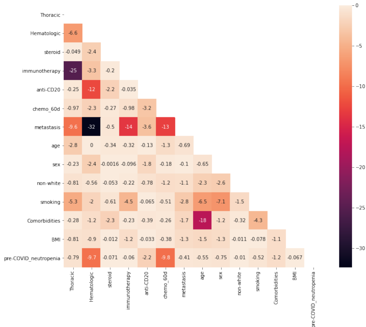
Figure S1. Pairwise Chi-square testing among variables. Values shown are \log_{10}(\text{p-value}) .
