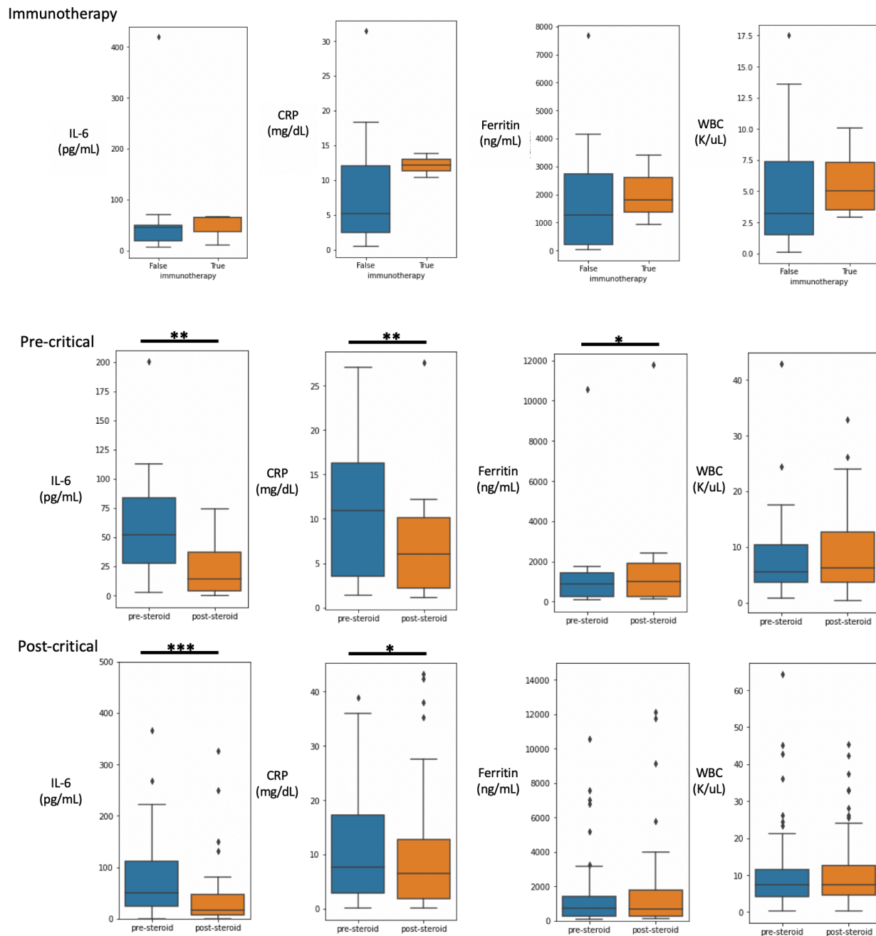
Figure S3. (Top) Boxplot showing quartiles and outliers of earliest laboratory values within 3 days of SARS-CoV-2 diagnosis for patients treated or not treated with immunotherapy 90 days prior. No comparisons were significant by Mann-Whitney U test with p-value cutoff of 0.05. Below, boxplots showing quartiles with outliers of paired laboratory values from prior to and after administration of high-dose corticosteroids (middle) prior to respiratory failure (nonrebreather,
