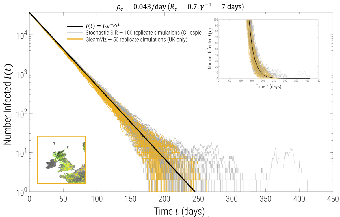
FIG. 1. Simulation trajectories on log-linear scale (inset: linear-linear scale) for a decay rate of \rho_e = 0.043/\text{day} , corresponding to R_e = 0.7 , 1/\gamma = 7 days, I_0 = 3.7 \times 10^4 and an initial recovered population of R(0) = 6 \times 10^6 . The solid black line is the deterministic prediction from Eqn.5, grey trajectories are 100 replicate Gillespie simulations of a standard SIR model, whilst the yellow trajectories are from 50 replicates using the spatial epidemic simulator GlemViz 17,18 restricted to the United Kingdom with a gravity model between heterogeneous sub-populations as shown in the inset map of the UK.
