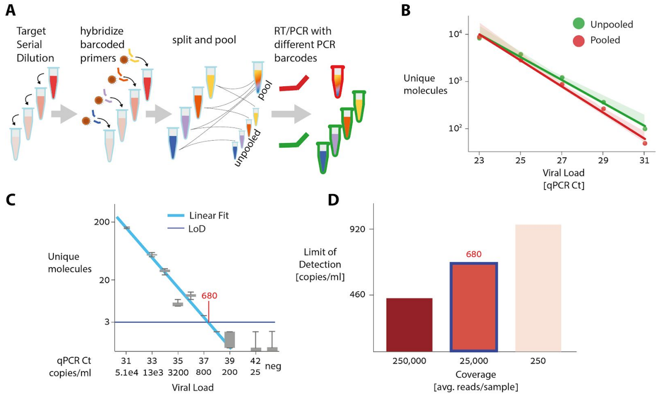
Figure 4: ApharSeq Sensitivity.
