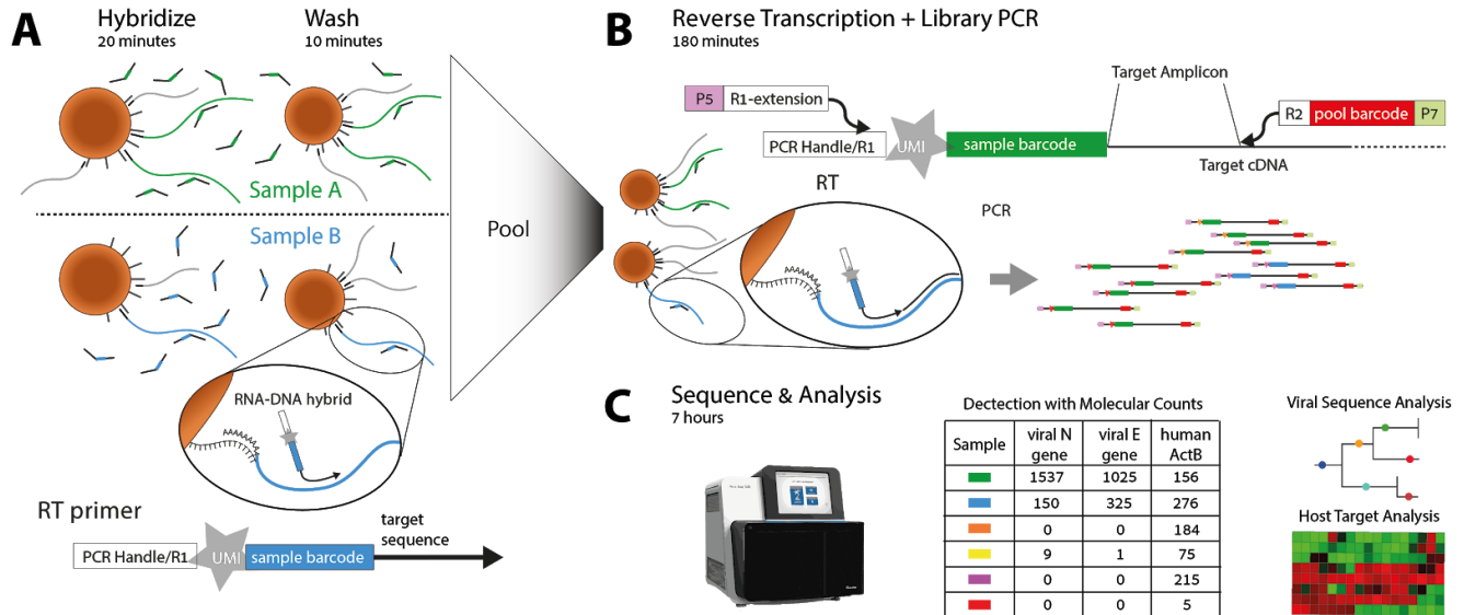
Figure 1 - ApharSeq overview
